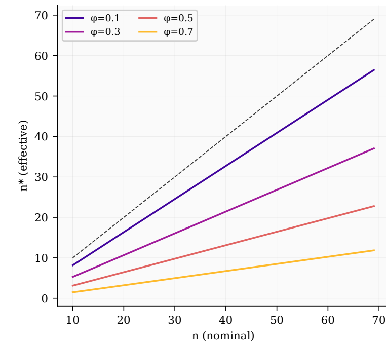
(f) Effective Sample Size
