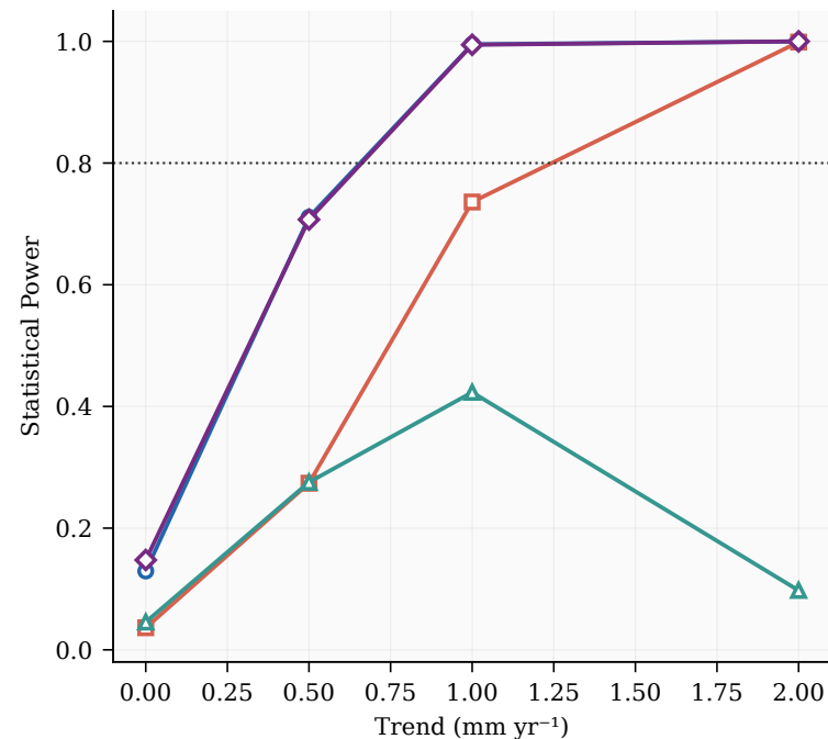
(b) Power ( \phi = 0.3 )
