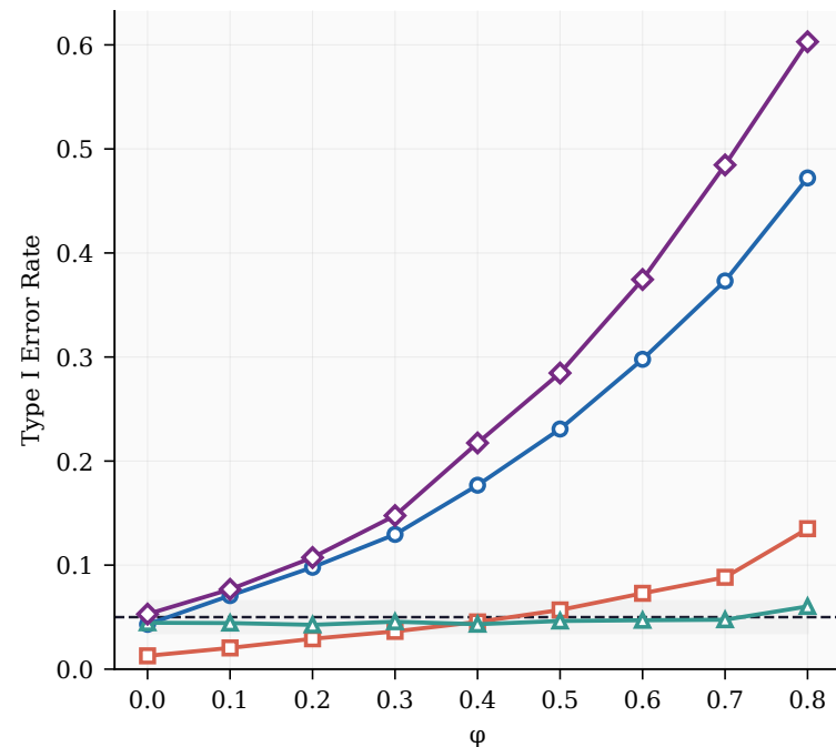
(a) Type I Error vs \phi
