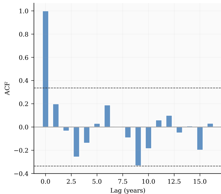
(e) ACF — Annual r_1=0.202 LB p=0.164
