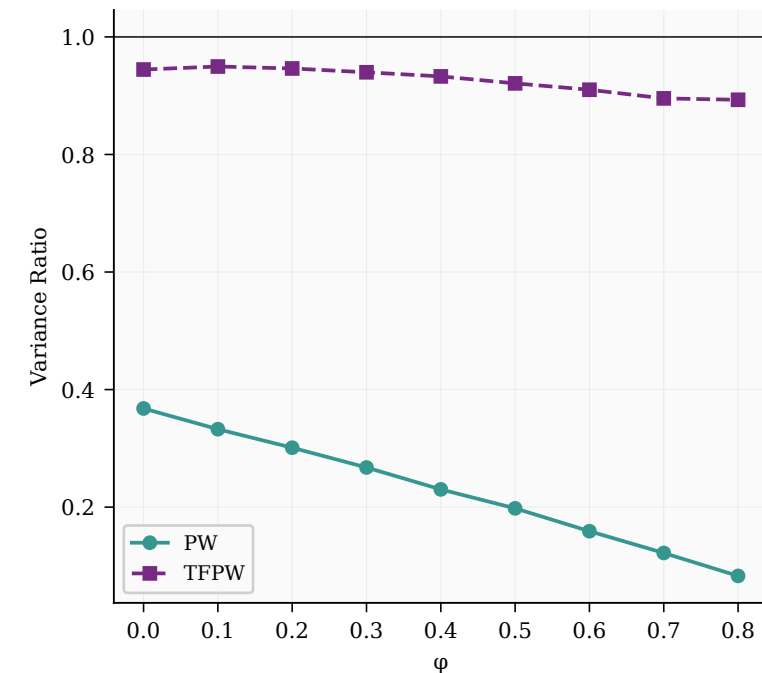
(c) Variance Distortion
