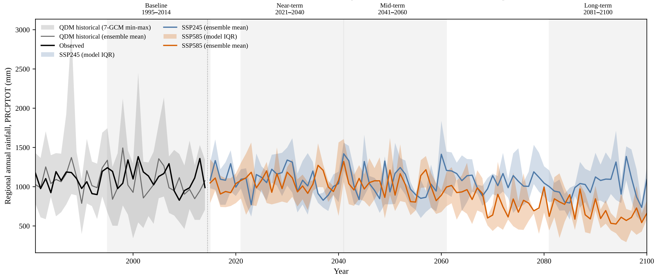
Uttaradit: observed and QDM bias-corrected CMIP6 regional rainfall with IPCC AR6 assessment periods
