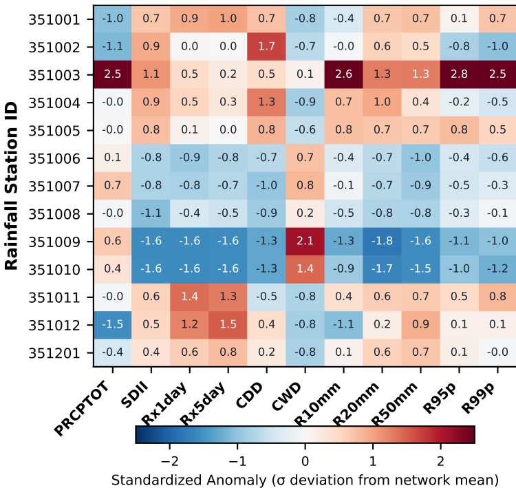
(a) Standardized ETCCDI Matrix (Z-scores, 1995-2014)
