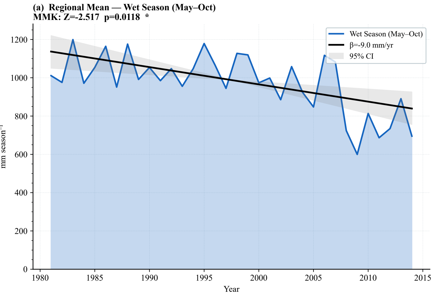
Figure 2. Hydrological Wet & Dry Season Rainfall Trend — 1981–2014 Wet: May–Oct | Dry: Nov–Apr | Modified MK + Sen's Slope
