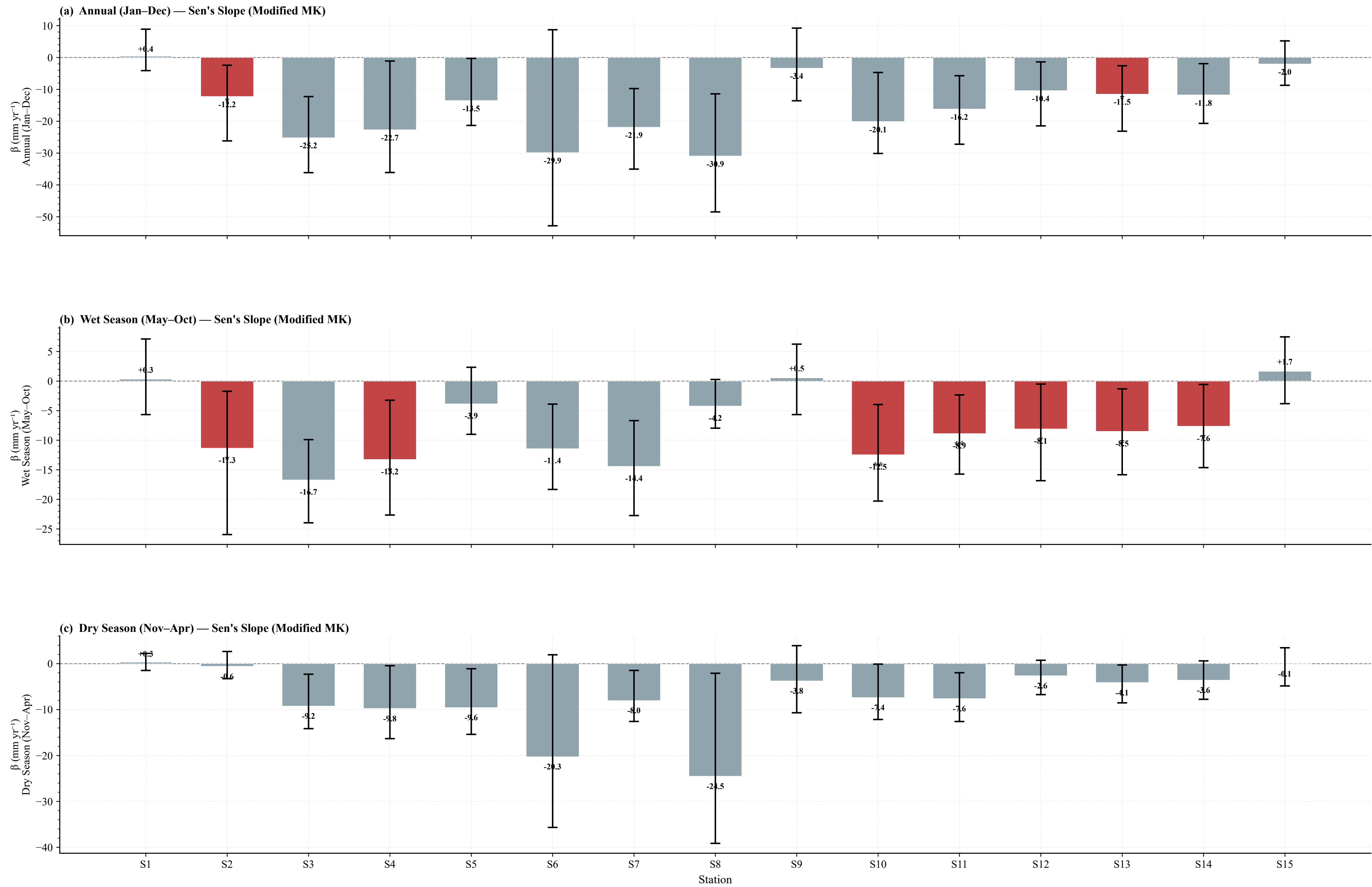
Figure 3. Sen's Slope Estimator — Annual, Wet, and Dry Season | 1981–2014 Error bars: 95% CI (Gilbert 1987) | * p<0.05 ** p<0.01
