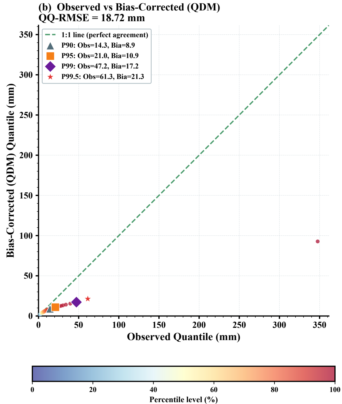
Figure 4 Quantile–Quantile plots comparing rainfall distributions between observed data and CMIP6 simulations before and after bias correction.
