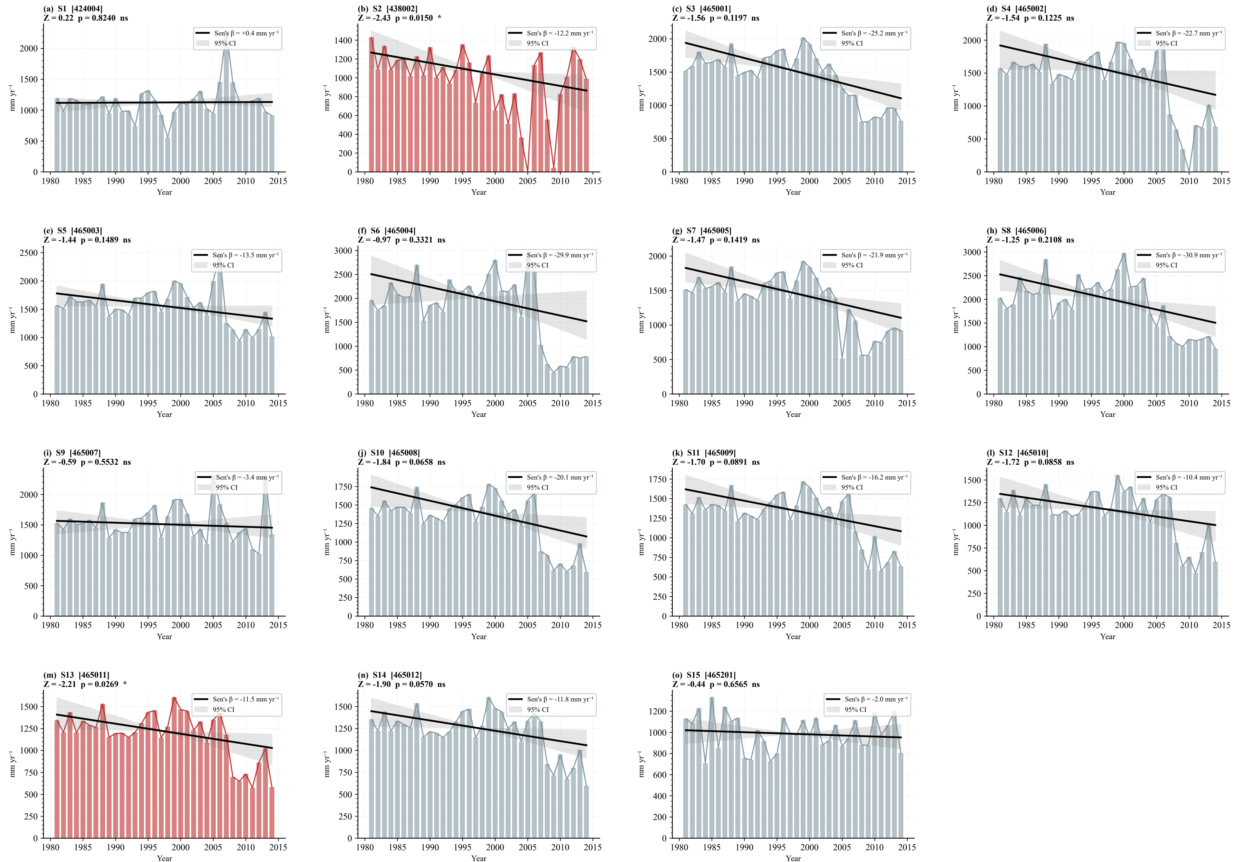
Figure 1. Annual Rainfall Time Series and Sen's Slope Trend — 1981–2014 Modified Mann–Kendall Test | * p < 0.05 ** p < 0.01 ns: not significant
