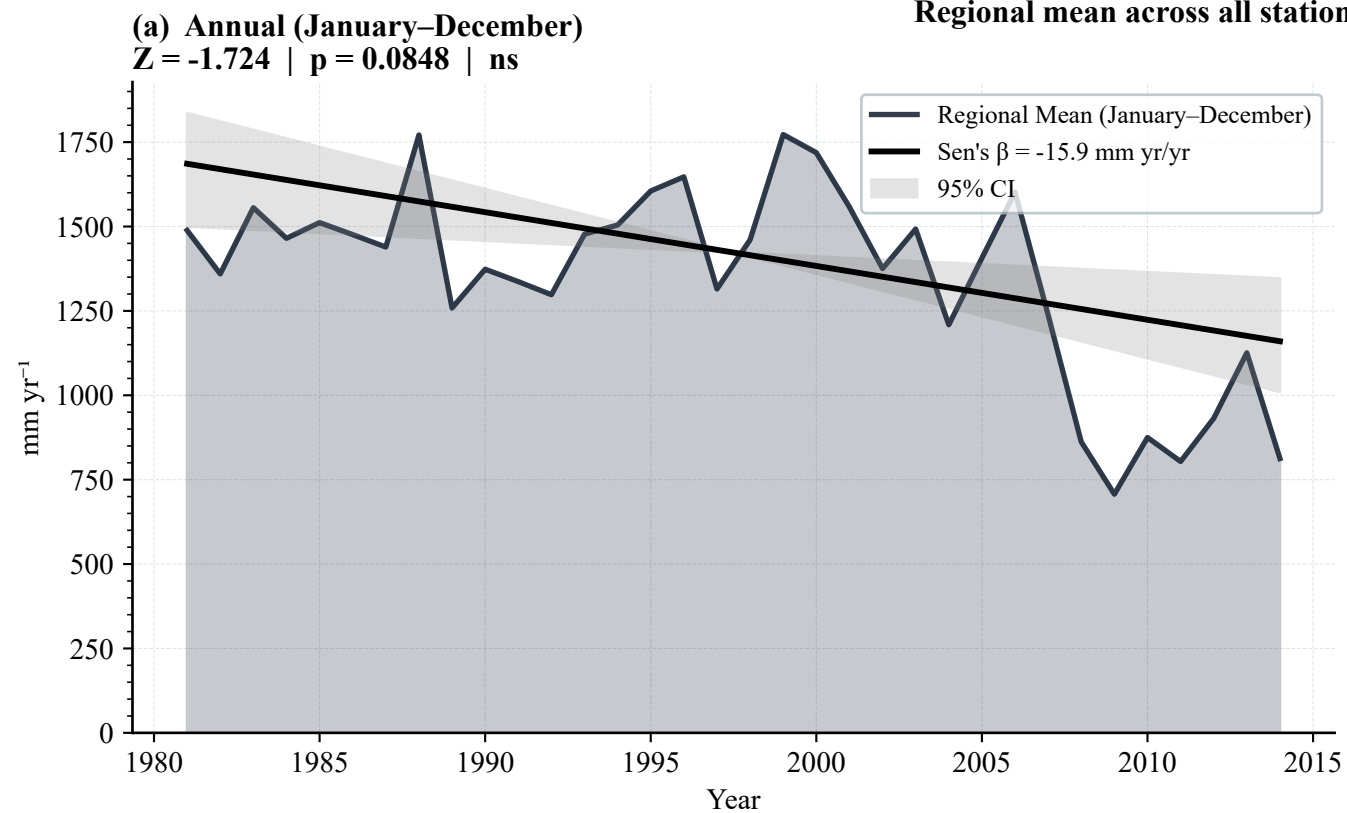
Figure 2. Seasonal Rainfall Time Series and Trend — 1981–2014 Regional mean across all stations | Modified Mann–Kendall Test + Sen's Slope
