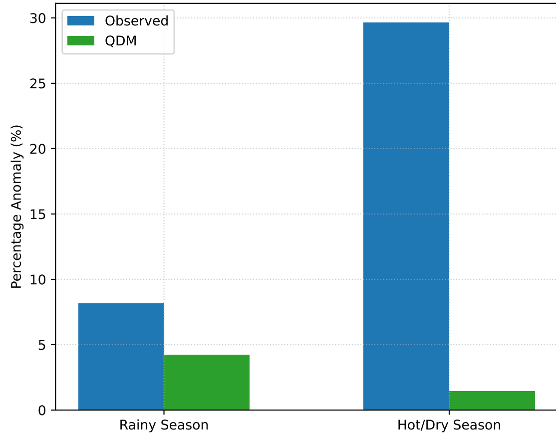
(b) Consecutive Wet Days (CWD)
