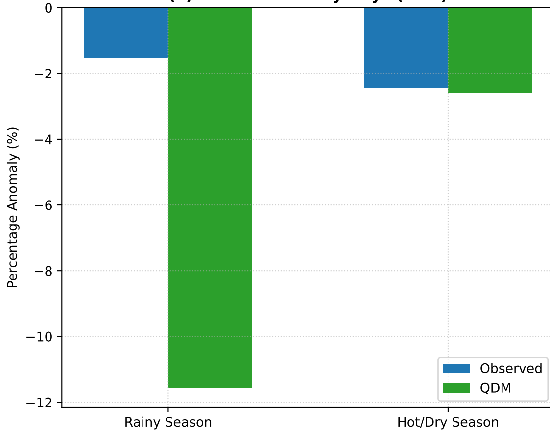
(a) Consecutive Dry Days (CDD)
