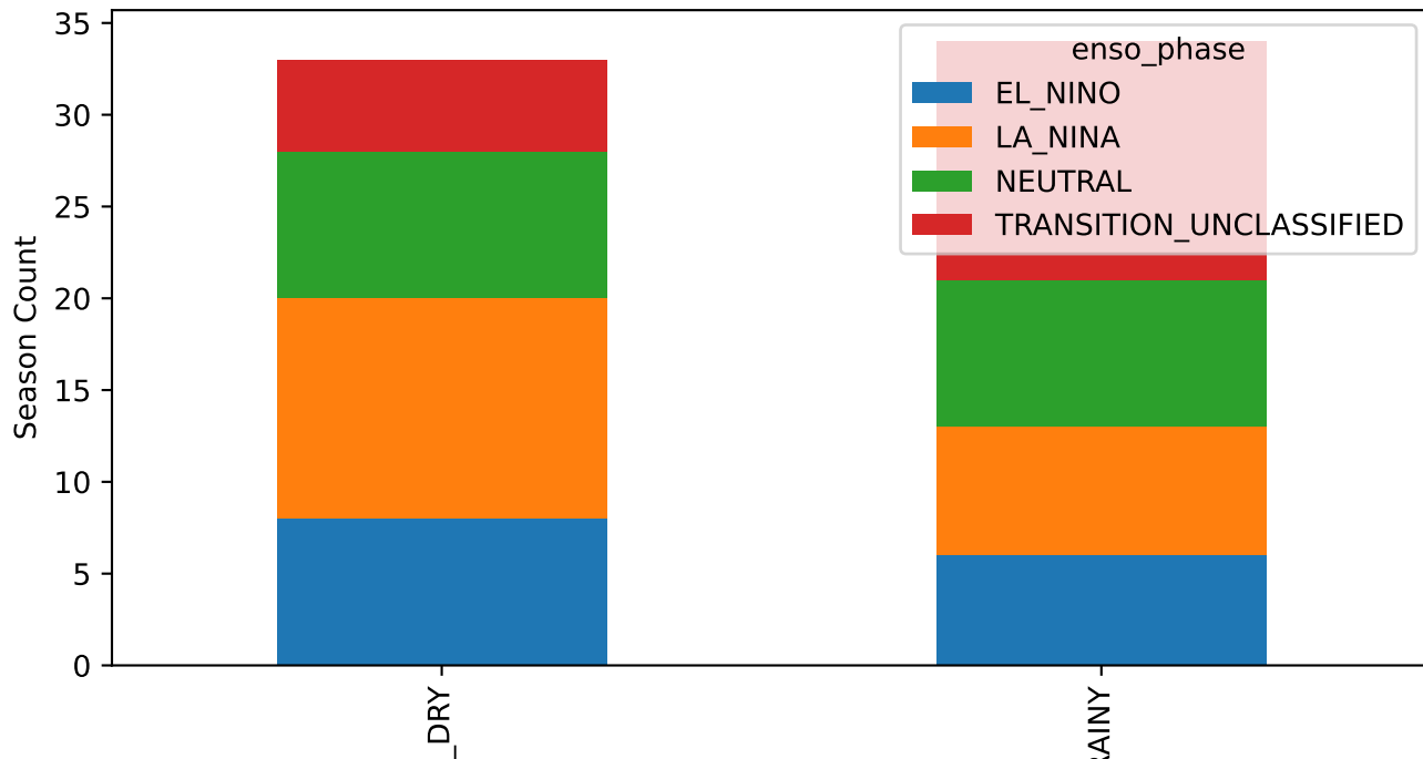
ENSO Sample Sizes - PrachuapKhiriKhan
