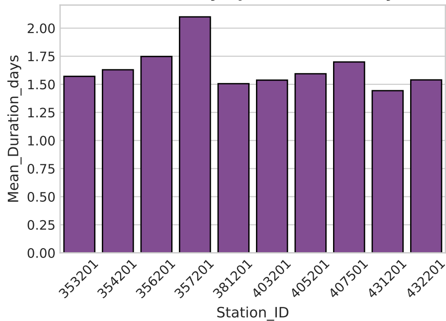
D. Mean Rainy-Spell Duration (days)
