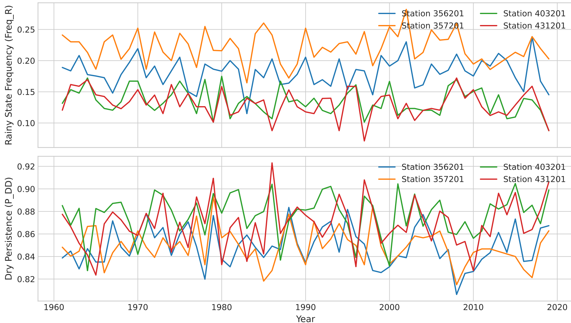
Figure 4. Long-Term Evolution of Rainy Frequency (A) and Dry Persistence (B) over 1961-2019
