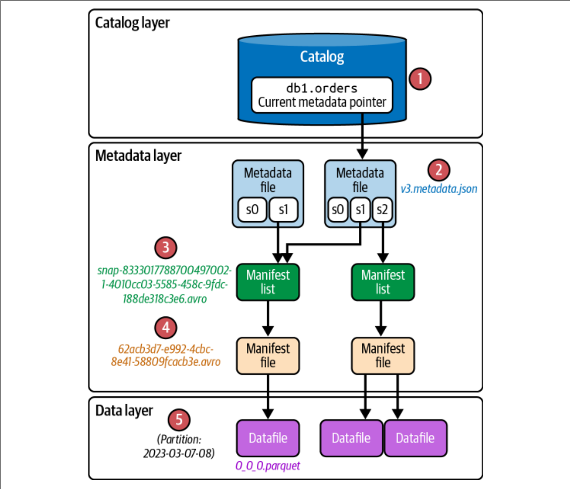
Figure 3-7. How the time-travel query works in Iceberg
