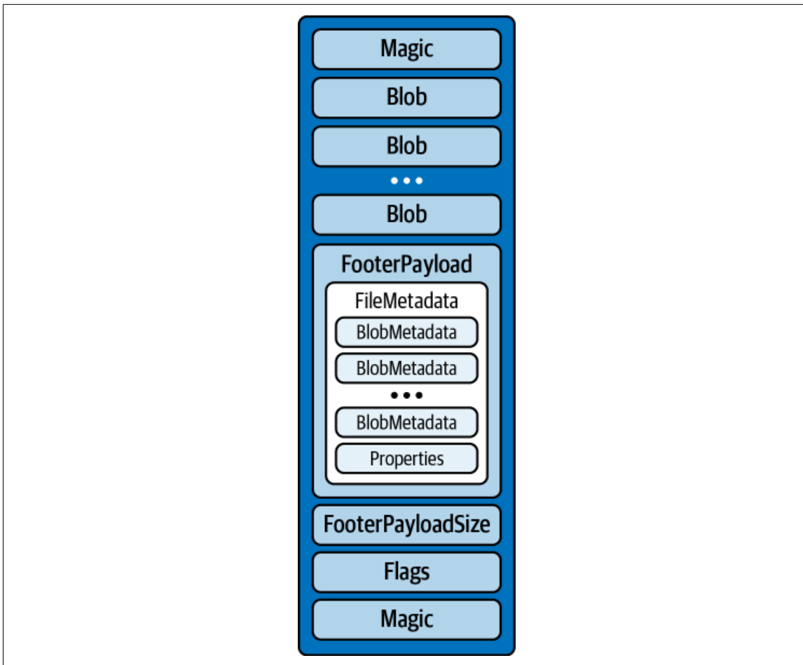
Figure 2-6. The structure of a puffin file
