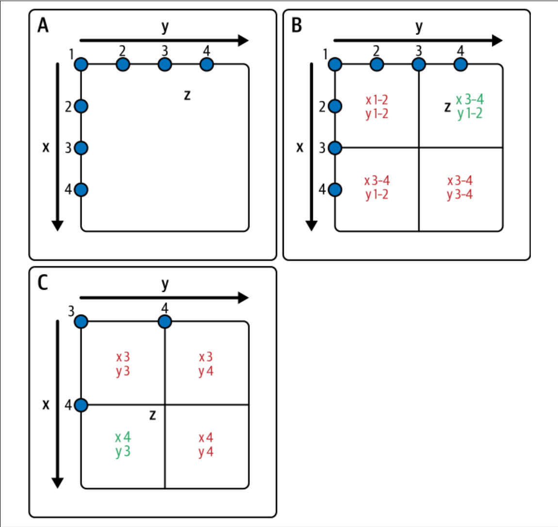
Figure 4-7. Understanding the basics of z-ordering
