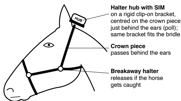
Halter hub with SIM on a clip-on bracket — crown piece, just behind the ears
