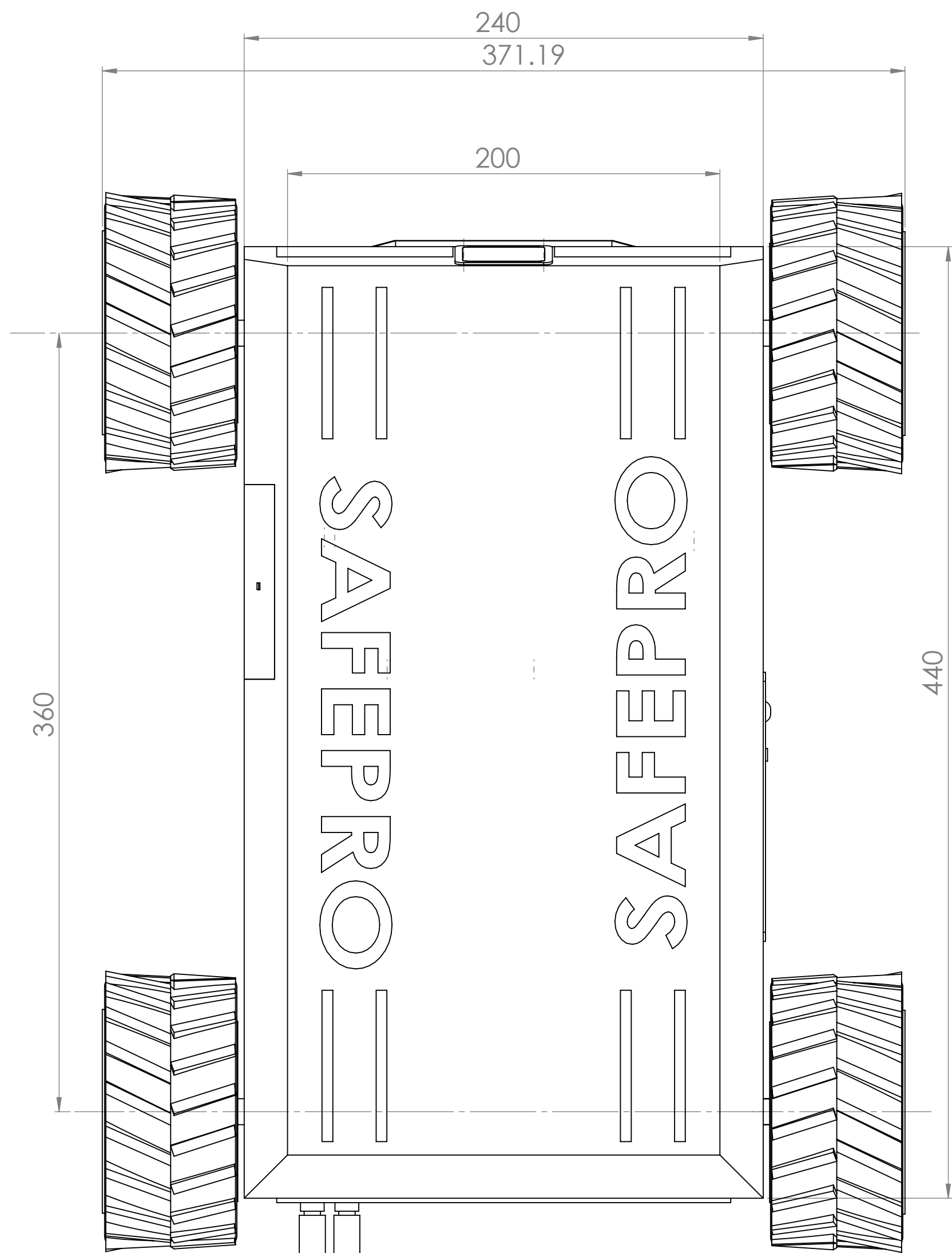
TOP VIEW
