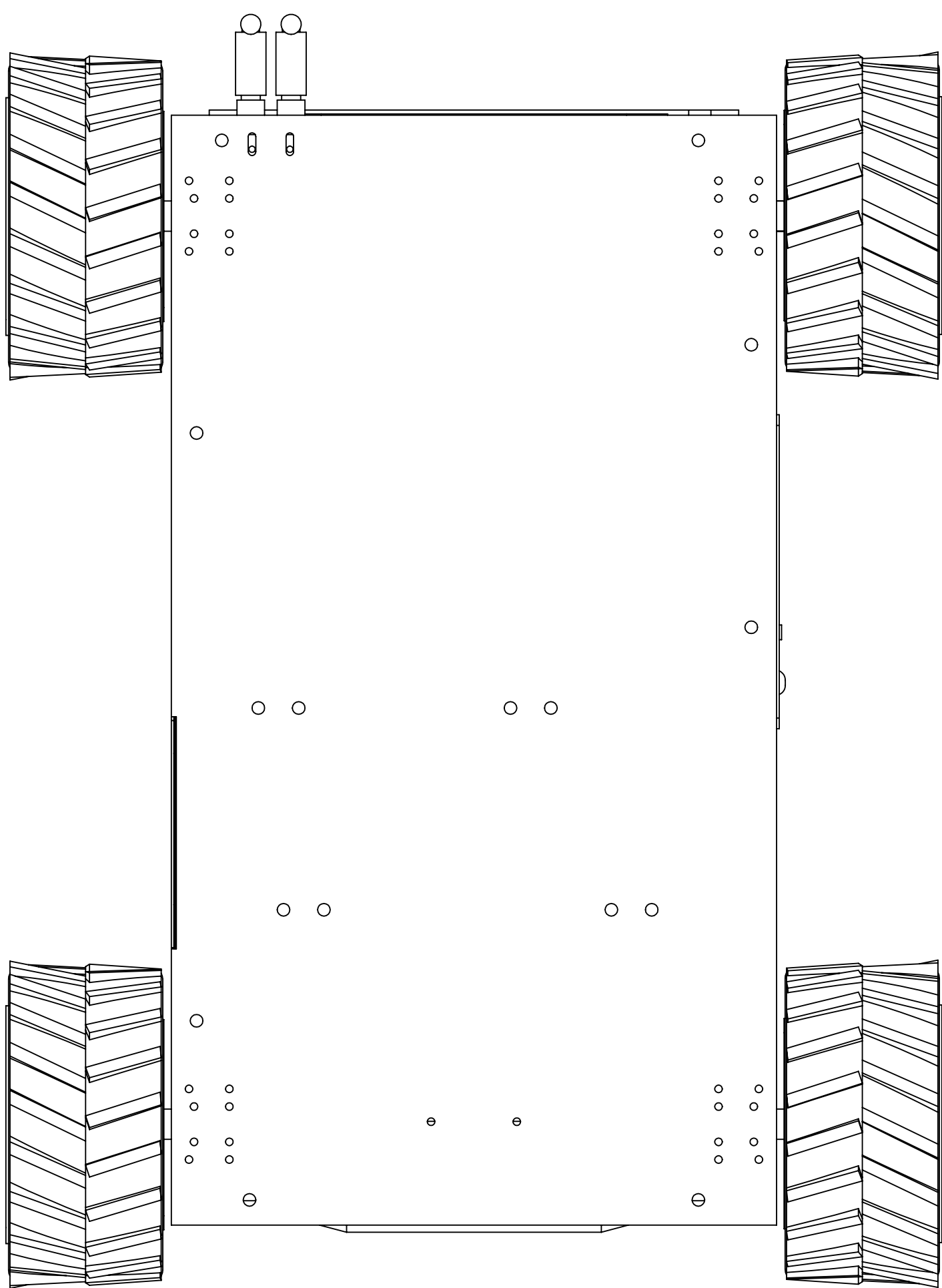
BOTTOM VIEW
