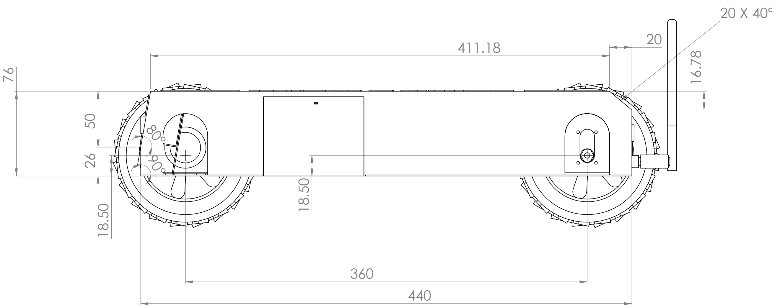
LEFT VIEW
