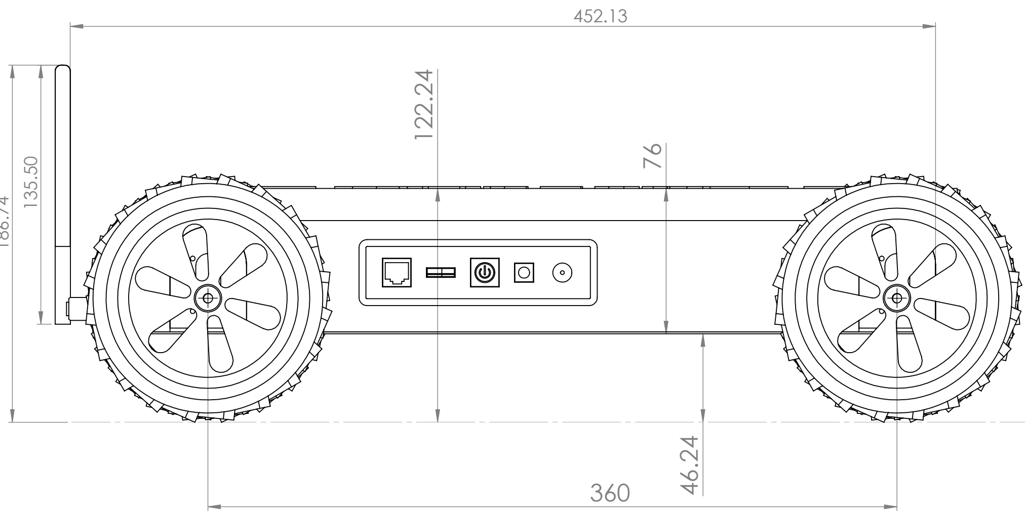
RIGHT VIEW
