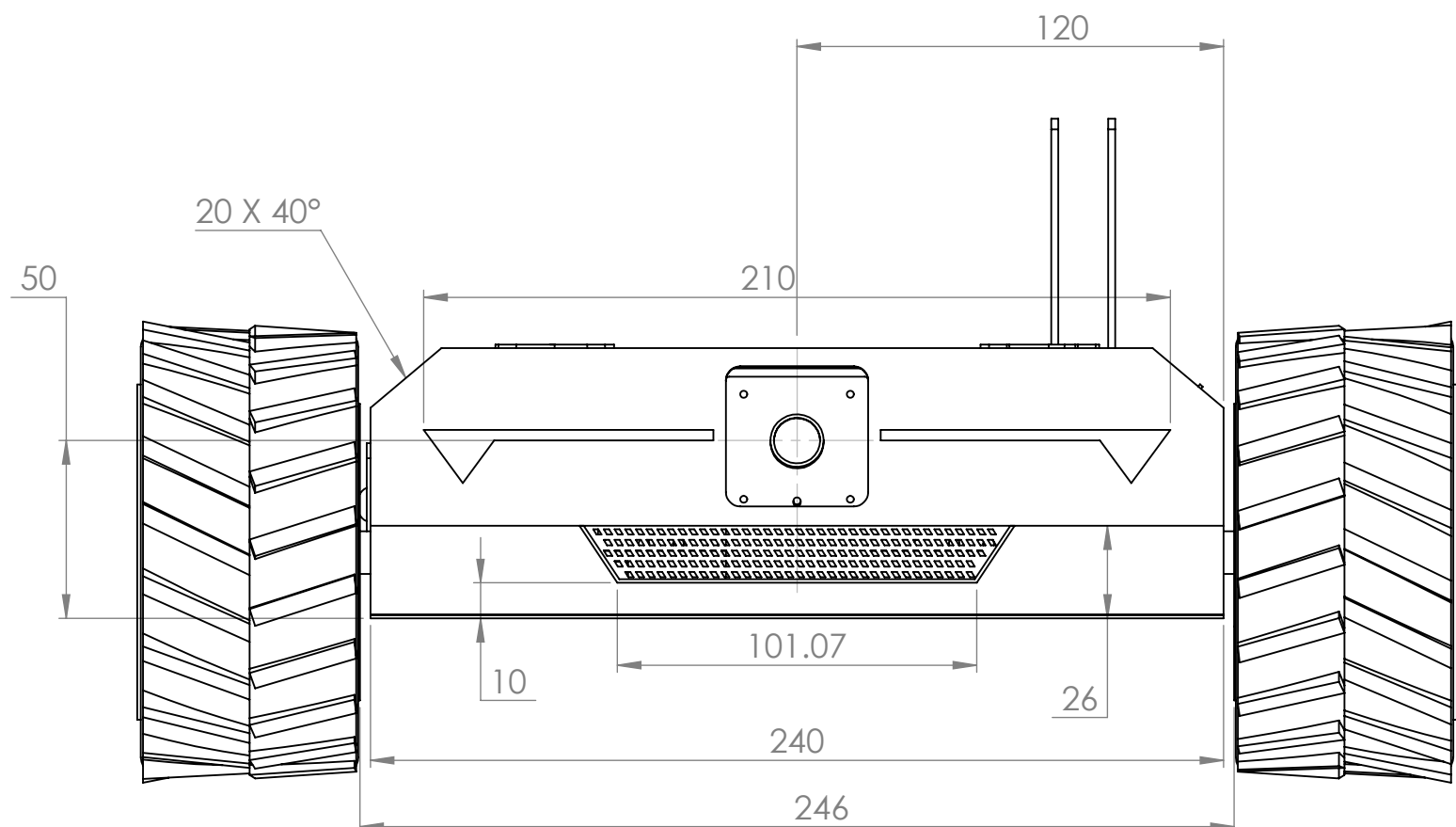
FRONT VIEW
