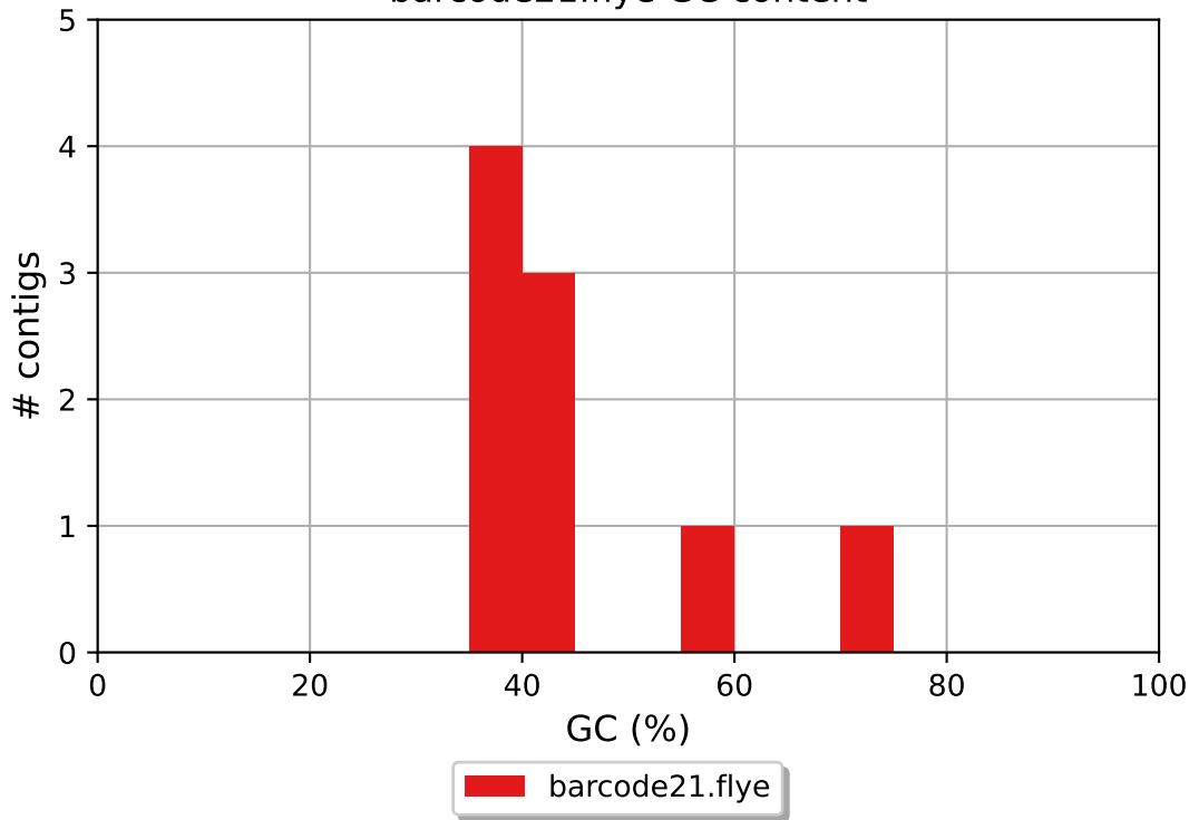
barcode21.flye GC content
