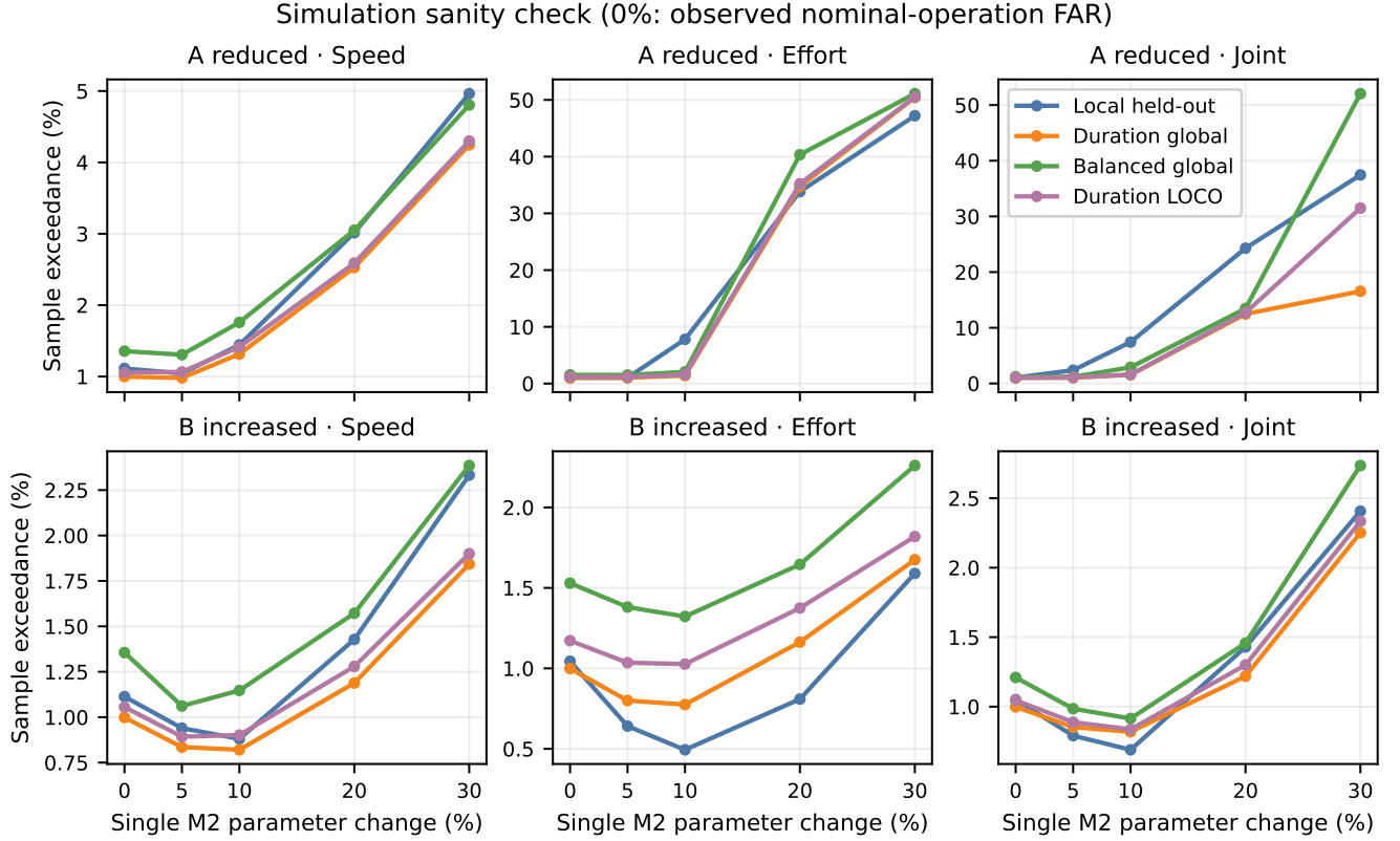
Fig. 7. Sample-weighted threshold-exceedance fractions for the two model-level changes. At 0% the plotted value is observed nominal-operation sample FAR; all positive-severity points are simulation-based.
