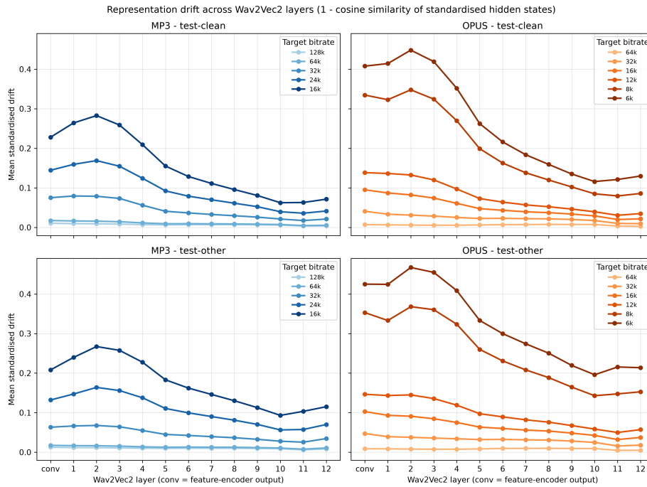
Figure 2. Mean standardised representation drift (1 – cosine similarity of per-dimension standardised hidden states; dimensionless) at the convolutional feature-encoder output (“conv”) and each transformer layer. Columns: MP3, Opus; rows: test-clean, test-other. Darker lines denote lower target bitrates. Means over 500 utterances.
