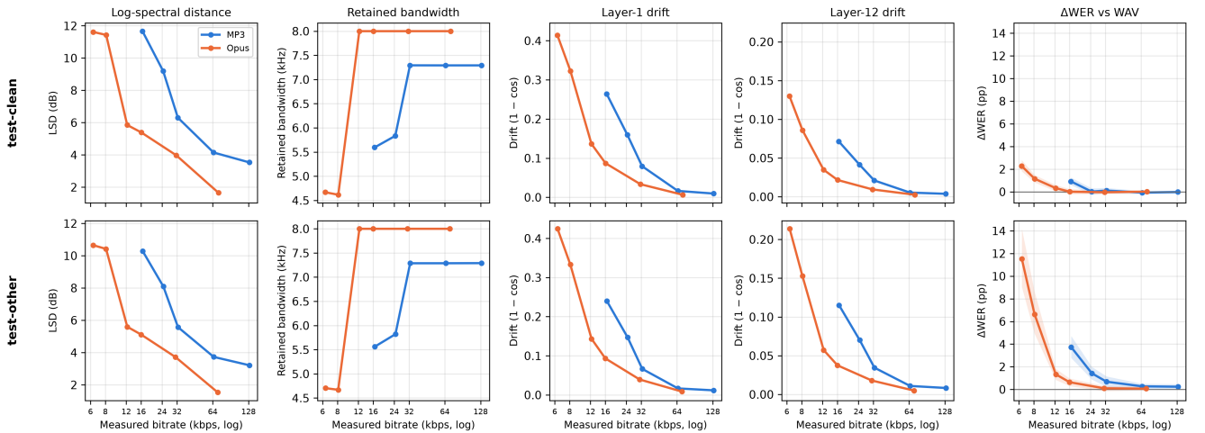
Figure 1. Signal, representation and recognition against measured bitrate (log scale) for MP3 (blue) and Opus (orange); top row test-clean, bottom row test-other. Columns: log-spectral distance (dB); retained bandwidth (kHz), the highest frequency at which the codec keeps power within 20 dB of WAV; standardised drift at layers 1 and 12 (1 – cosine similarity, dimensionless); \Delta WER relative to WAV (percentage points; shaded: 95% speaker-level bootstrap CI). Each point is a mean over 500 utterances.
