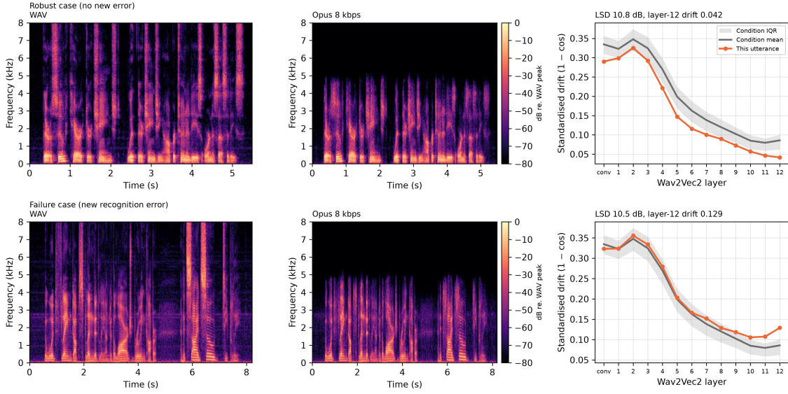
Figure 4. Robust versus failure case at Opus 8 kbps (test-clean), selected by the rule in Section 3.7. Left, centre: spectrograms (dB relative to the WAV peak; frequency in kHz, time in s) of the WAV and decoded signals; both lose content above about 4.5 kHz. Right: the utterance’s standardised drift profile (orange) against the condition mean and interquartile range (grey). Robust case 7729-102255-0025: LSD 10.8 dB, layer-12 drift 0.042, transcript unchanged. Failure case 672-122797-0073: LSD 10.5 dB, layer-12 drift 0.129, “FLAMED UP” recognised as “FLAME OT”.
