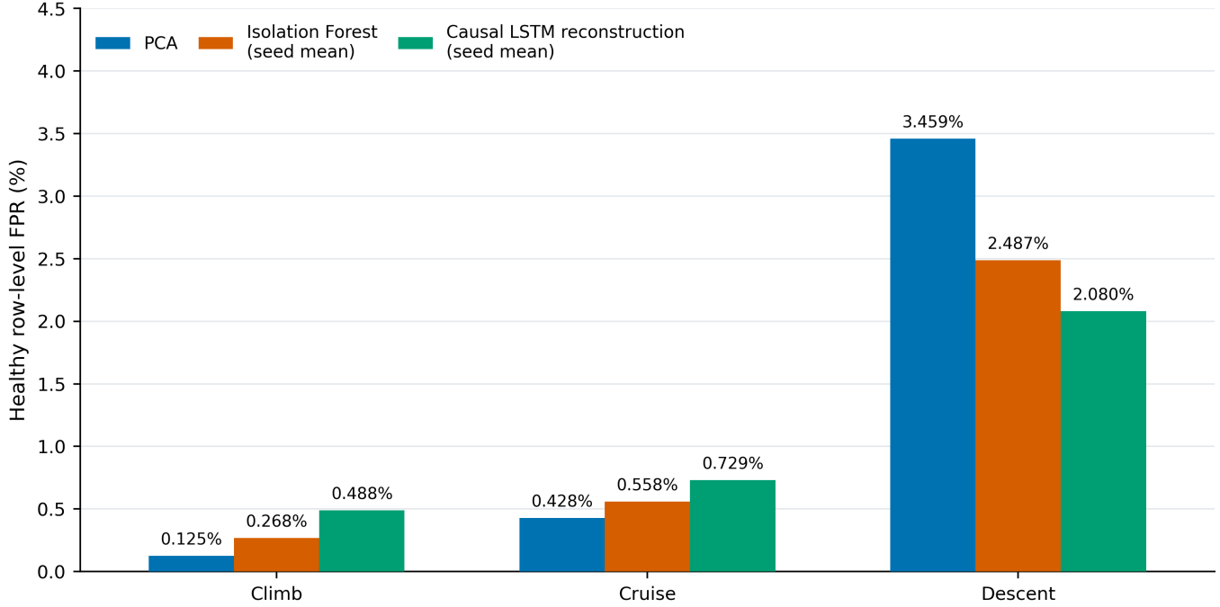
Fig. 2. DS02 exploratory healthy row-level FPR at the nominal 1% pooled calibration target. PCA is a single run; Isolation Forest and the causal LSTM sequence-reconstruction network are arithmetic three-seed means. Bars show pooled-threshold phase FPR, not cross-phase transfer FPR. Figures 2 and 4 use the same vertical scale to support direct visual comparison.
