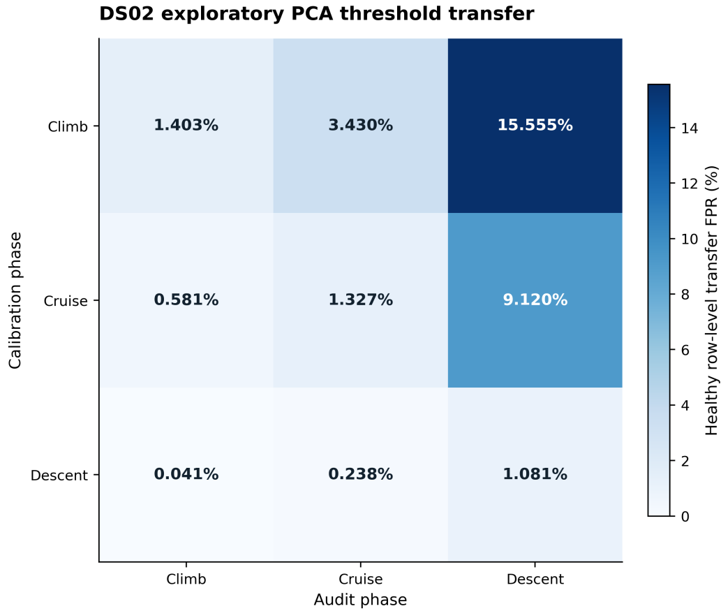
Fig. 3. DS02 exploratory PCA cross-phase threshold transfer at the nominal 1% target. Calibration phase is shown vertically and healthy audit phase horizontally. Each cell is the held-out transfer FPR after phase-specific calibration, not pooled phase FPR. Diagonal cells are same-phase audit FPRs and are not constrained to exactly 1%.
