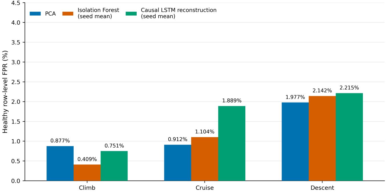
Fig. 4. DS03 frozen confirmatory healthy row-level FPR at the nominal 1% pooled calibration target. PCA is a single run; Isolation Forest and the causal LSTM sequence-reconstruction network are arithmetic three-seed means. Bars show pooled-threshold phase FPR, not cross-phase transfer FPR. The vertical scale matches Fig. 2; no seed-mean confidence interval was executed.
