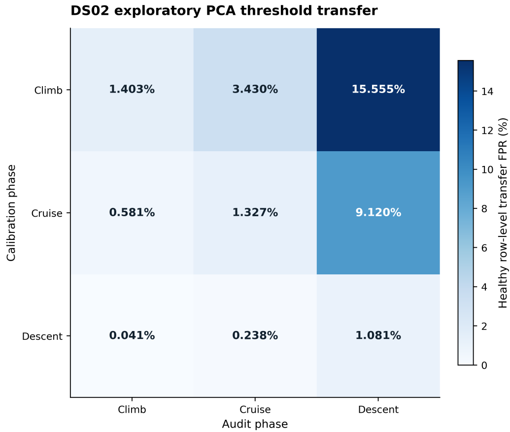
Fig. 3. DS02 exploratory PCA cross-phase threshold transfer at the nominal 1% target. Calibration phase is on the vertical axis and healthy audit phase on the horizontal axis. Each cell is transfer FPR after phase-specific calibration, not pooled-threshold phase FPR. PCA has no seed mean. Diagonal cells are held-out same-phase audit FPRs and are not constrained to exactly 1%. Values are cross-phase transfer FPRs, not pooled phase FPRs.
