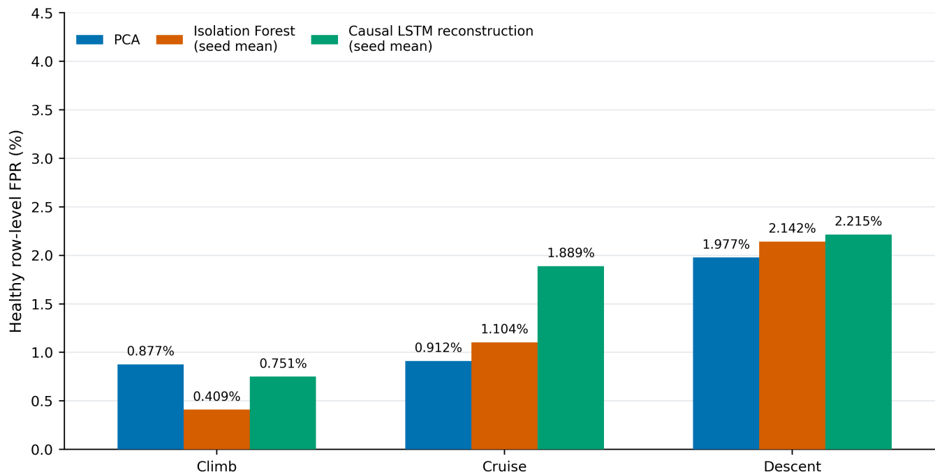
Fig. 4. Frozen DS03 confirmatory phase-wise healthy row-level FPR at the nominal 1% pooled calibration target. PCA is a single run; Isolation Forest and causal LSTM reconstruction are arithmetic three-seed means. Bars are pooled-threshold phase FPRs, not cross-phase transfer FPRs. The vertical scale matches Fig. 2. Error bars are omitted because run-level and seed-mean uncertainty are not interchangeable; no hierarchical-bootstrap interval for either seed mean was executed.
