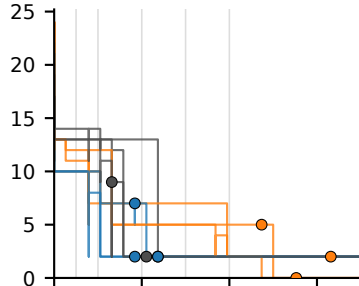
Past-only LSTM
