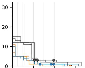
Isolation Forest
