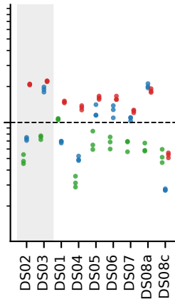
Past-only LSTM
