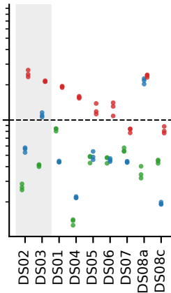
Isolation Forest
