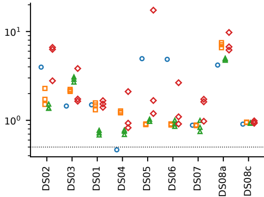
Worst-engine max |FPR - \alpha| (P)
