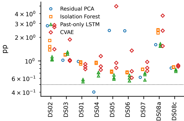
Mean per-engine max |FPR - \alpha| (P)
