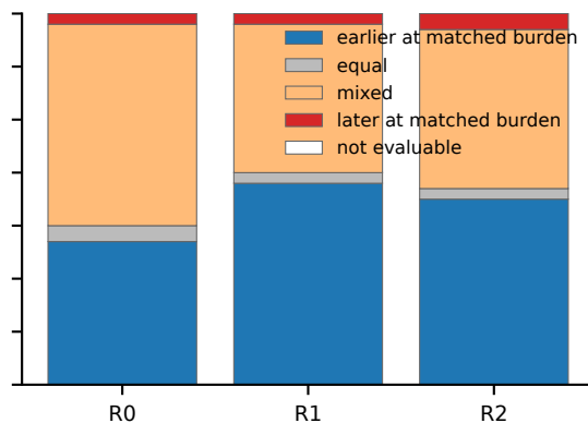
Q vs P (all new-subset runs, \alpha = 1\% )
