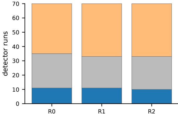
C vs P (all new-subset runs, \alpha = 1\% )
