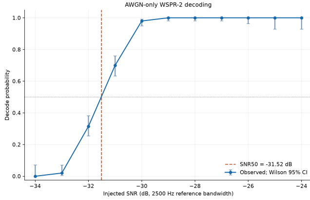
FIGURE 1. AWGN-only production- w_{sprd} P_{decode} versus injected SNR (dB, 2500-Hz reference), with Wilson intervals and an interpolated 50% point.
