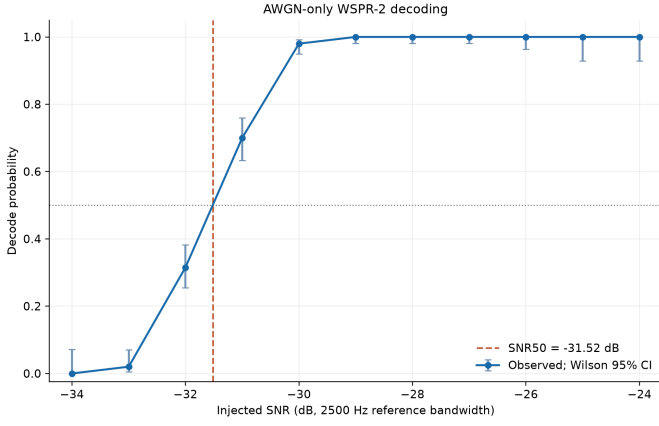
Fig. 1. AWGN-only production-wsprd P_{\text{decode}} versus injected SNR (dB, 2500-Hz reference), with Wilson intervals and an interpolated 50% point.
