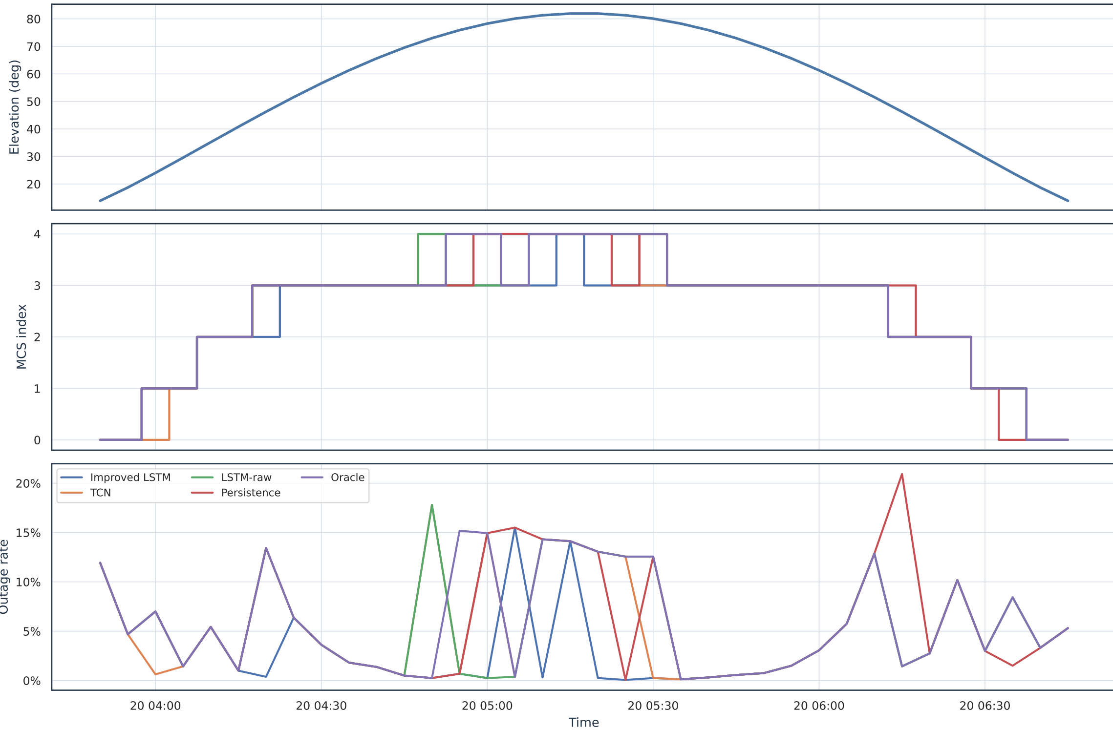
Example pass geometry and policy behavior
