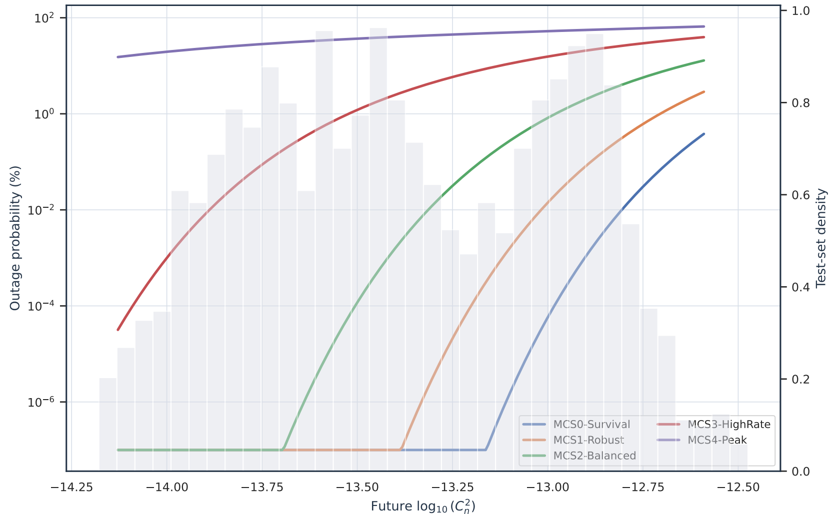
Turbulence-to-link response curves
