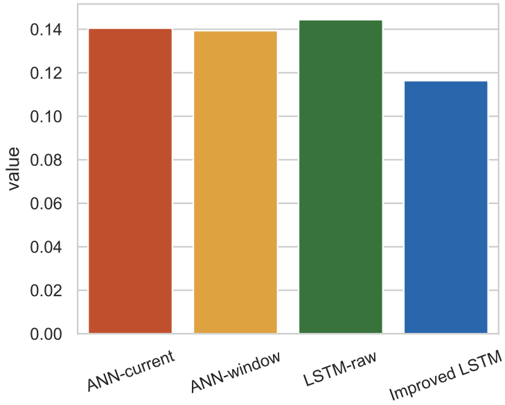
RMSE
