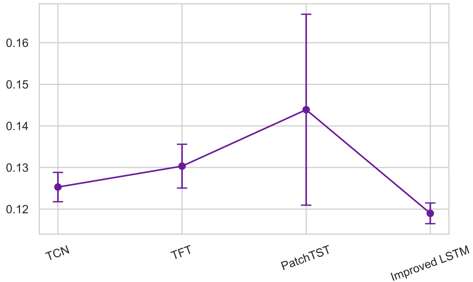
RMSE (mean \pm std)
