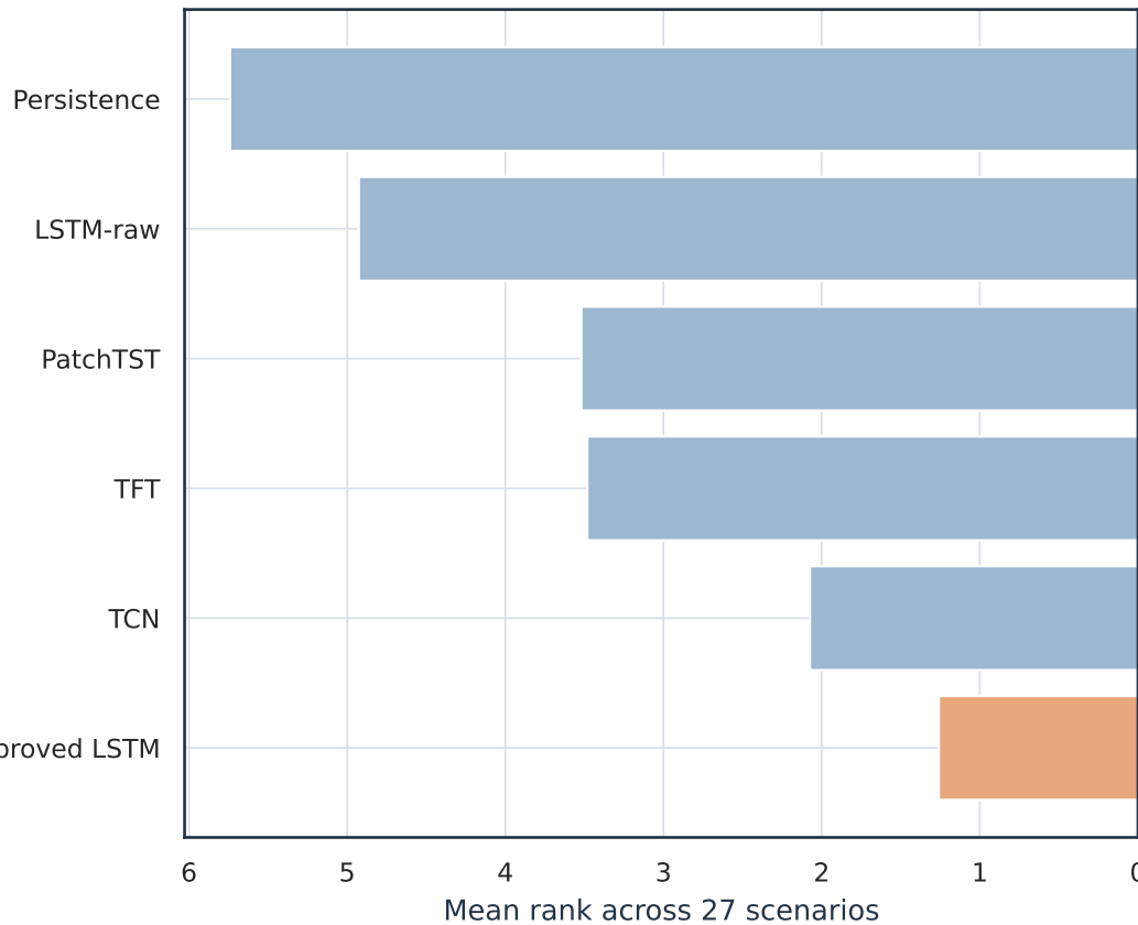
Rank stability
