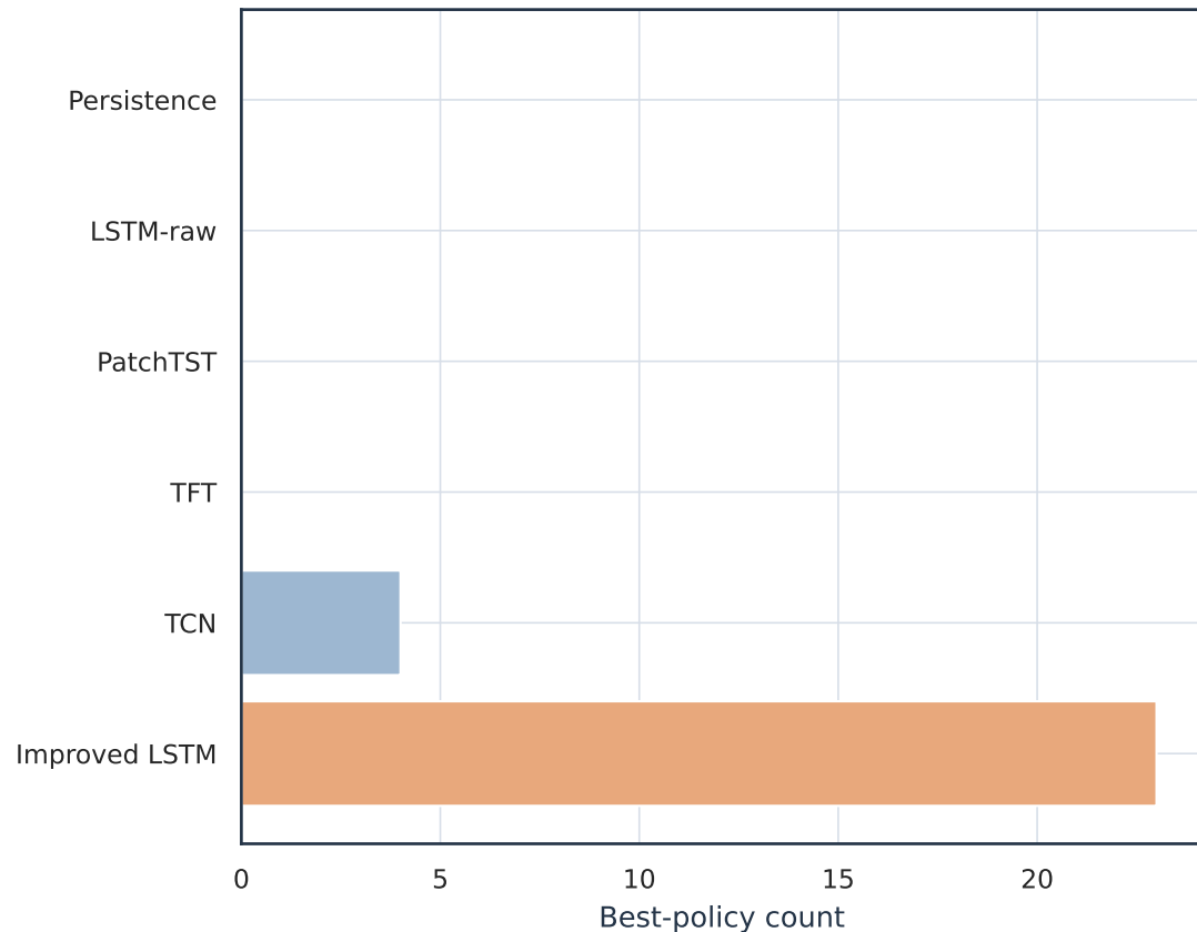
Scenario wins
