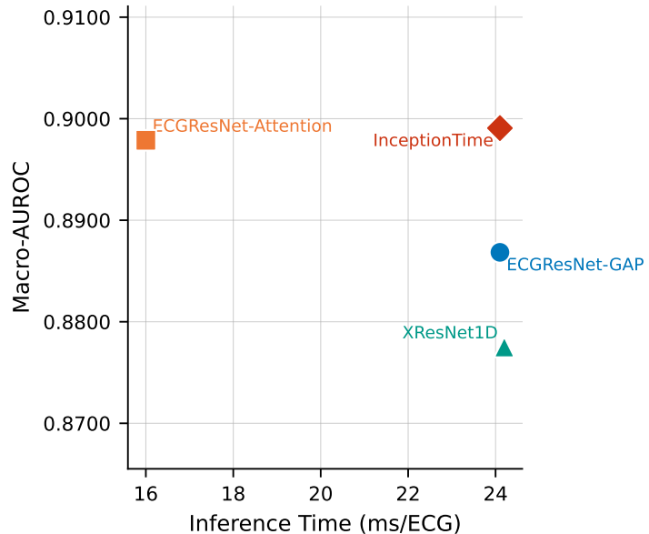
(B) Macro-AUROC vs. Inference Time
