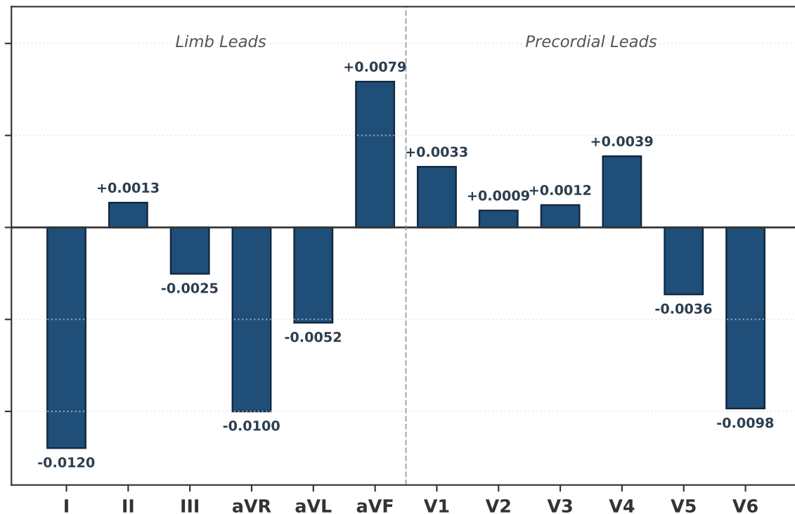
(B) InceptionTime (Baseline AUROC = 0.7899)
