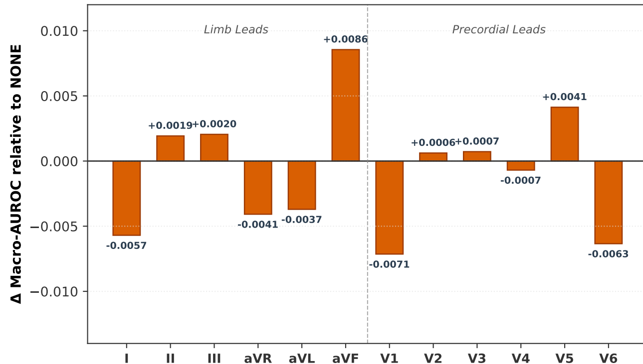
(A) ECGResNet-GAP (Baseline AUROC = 0.7682)
