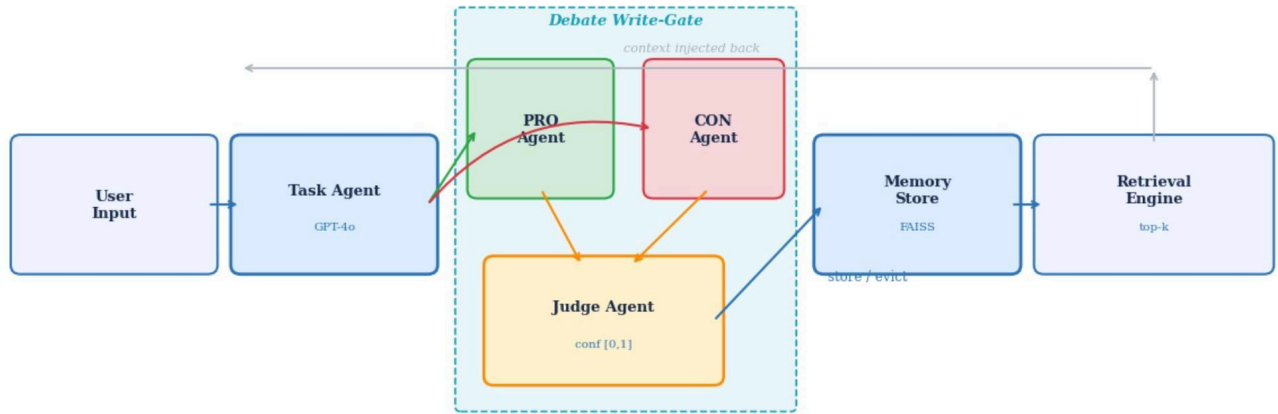
Figure 1: MemDebate system architecture. Every claim from the Task Agent passes through the Debate Write-Gate before any memory write is performed. The Judge’s confidence score also drives retrieval ranking.
