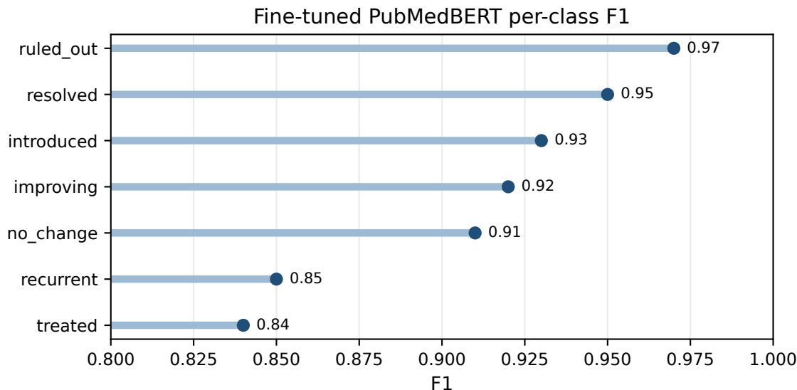
Figure 4: Per-class F1 for fine-tuned PubMedBERT.
