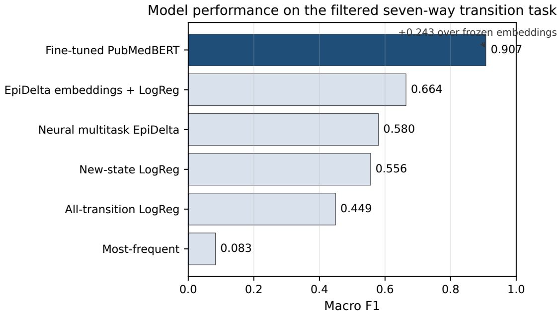
Figure 1: Model comparison on the filtered seven-way MedEST transition task.
