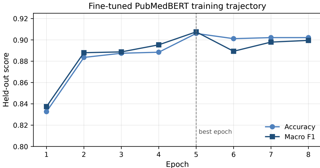
Figure 2: Fine-tuned PubMedBERT training trajectory. The best checkpoint occurs at epoch 5.
