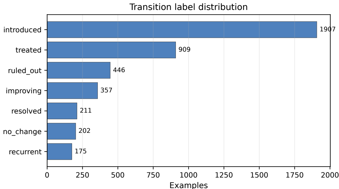
Figure 3: Filtered transition label distribution. The task is imbalanced, motivating macro F1 as the primary metric.
