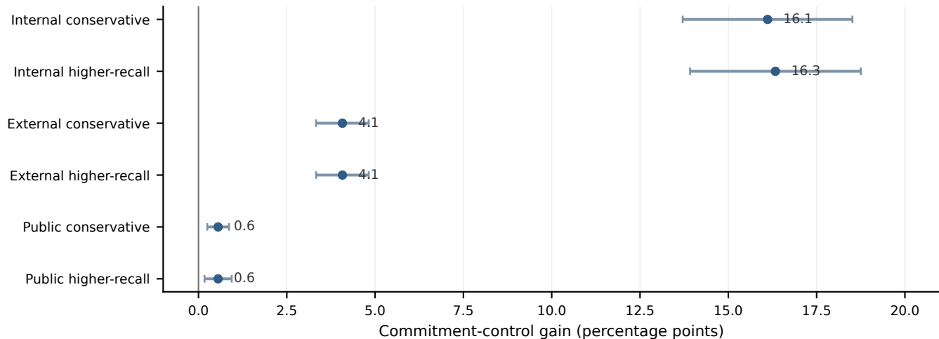
c Paired commitment-control gain
