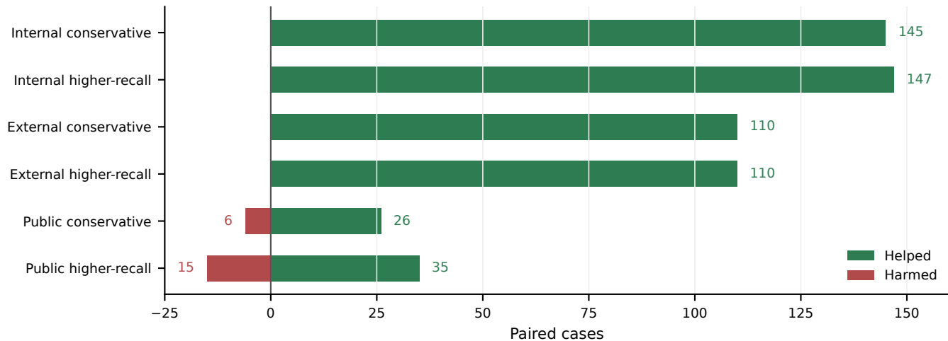
c Paired commitment-control gain
