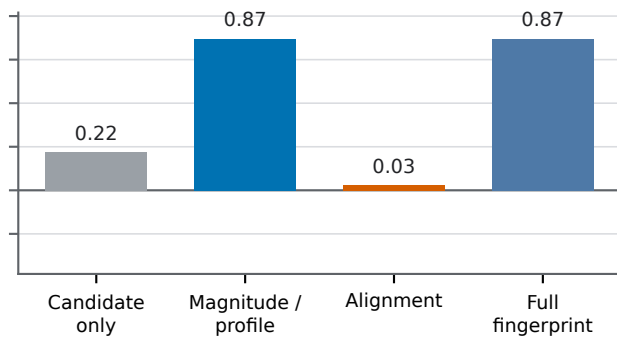
Qwen/RippleEdits · known-protected damage
