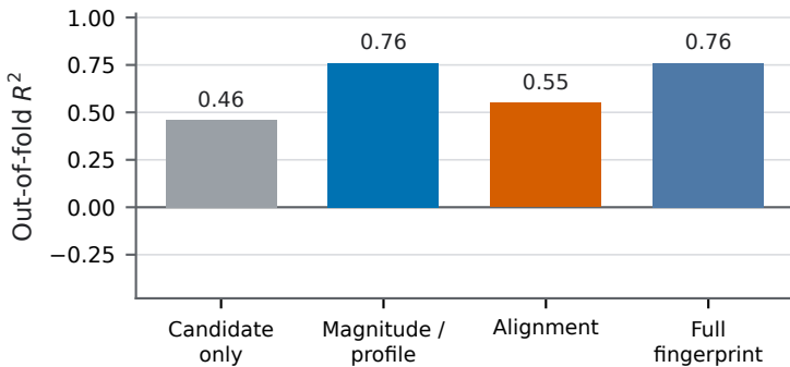
Controlled GPT-2 · protected damage
