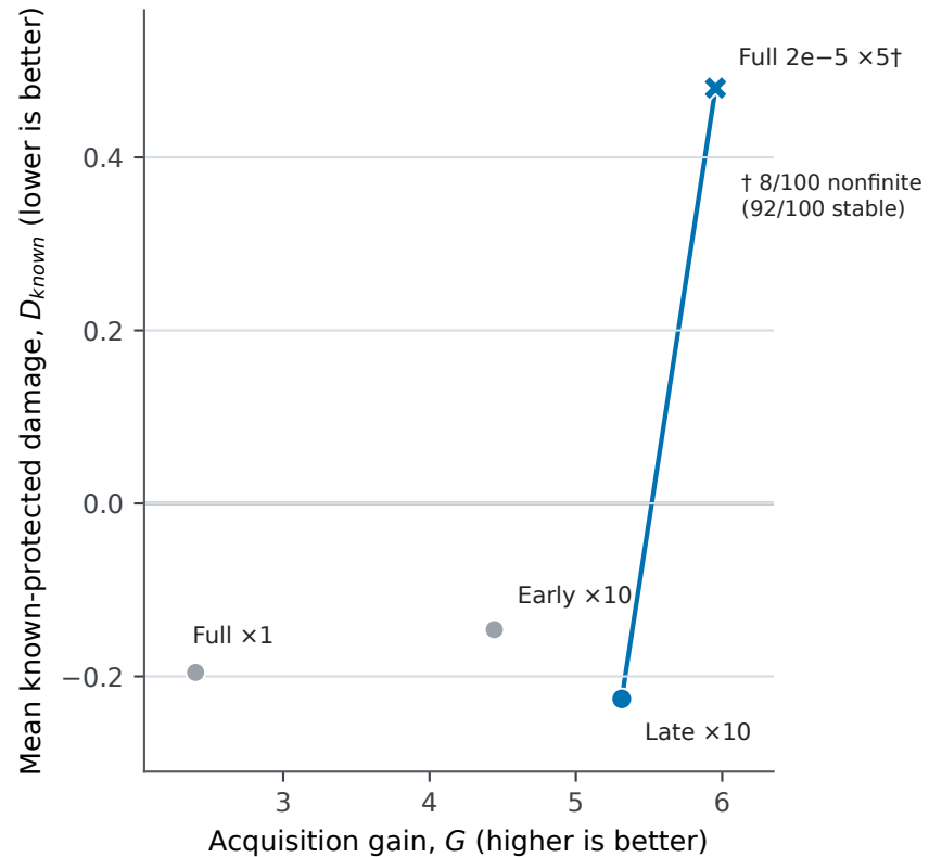
Qwen2.5-0.5B / RippleEdits (100 edits)
