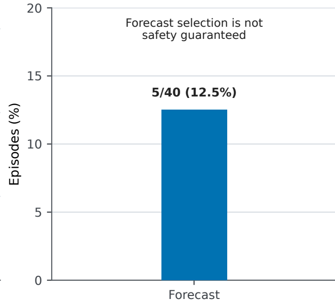
Constraint-violation rate
