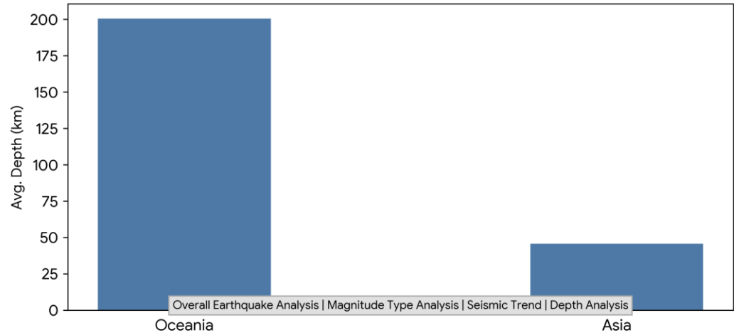
Earthquake Depth Analysis Storyboard
