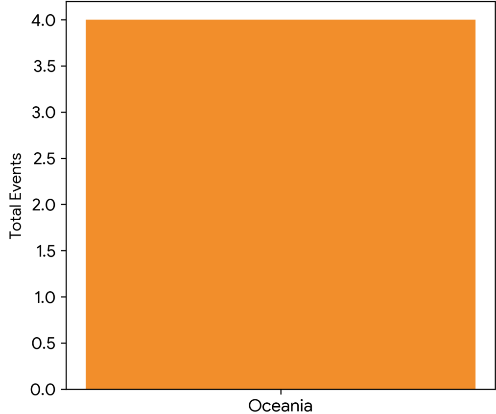
Earthquake Comparison (Filtered: Oceania)
