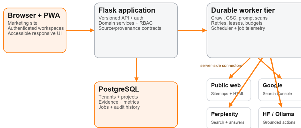
Figure 1 — Target production architecture. The current monolith is refactored behind the same product contract.
