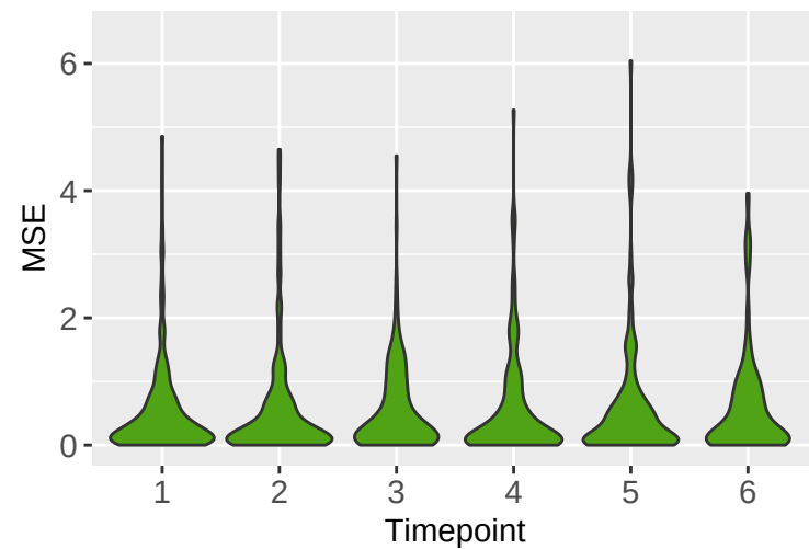
Training T6
