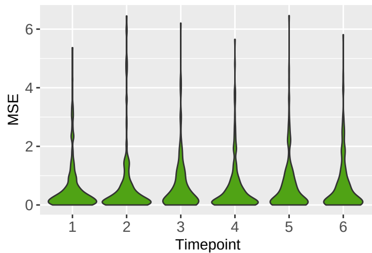
Training T5
