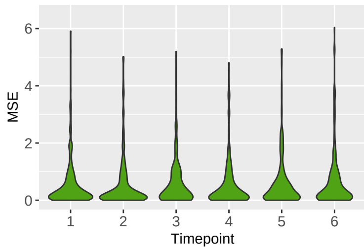
Training T4
