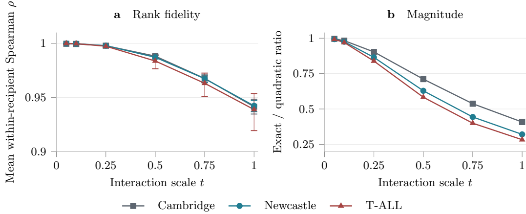
Fig. 3 The response ranking remains stable from independence to the fitted interaction. a , Mean within-recipient Spearman correlation between the local response coefficient and exact finite-strength model discrepancy; lines show recipient-bootstrap 95% intervals. b , Ratio of summed exact discrepancy to the quadratic approximation. Exact discrepancy is twice the forward KL divergence from the recipient covariance reconstruction to the cohort-pool reconstruction. All points use the same 95 recipients, 81 queries, assay marginals, and source interaction as the primary analysis.
