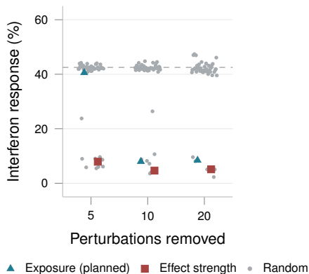
c Removing training perturbations
