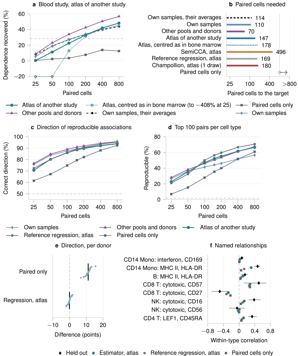
Fig. 2 An atlas from another study reduces the number of paired cells a new blood study needs. a , Validation test (prespecified): fraction of the dependence within broad cell types recovered in a held-out sample against the number of paired cells, drawn from two other samples of its processing pool and centred by contrasts, pooled over 34 held-out samples. Unpaired cells came from an atlas of another study, the study's other pools and donors, or the paired samples themselves; two further lines centre the paired cells on averages from the unpaired cells of the same samples or, with the atlas, on the drawn paired cells' own averages, as in the bone-marrow test. Dashed line, the accuracy target (half the best recovery); values below -20\% are drawn at -20\% . b , Paired cells needed to reach the target, including three other methods given the same paired cells and atlas (follow-up; Champollion on one draw of five); arrow, not reached within 800. c , Follow-up readout: fraction of the held-out sample's reproducible associations (same sign in both halves of its cells, with P < 0.01 in each; 3.2% of gene-protein pairs) whose direction the estimate predicted correctly; dashed line, guessing. d , Fraction of the 100 pairs with the largest absolute estimated correlations in each held-out sample and cell type that were reproducible associations with the predicted sign; dashed line, random pairs. In c and d , paired-only estimation and reference regression are each the best of their methods or forms at each budget. e , Per donor (points), the atlas estimate's share of correct directions with 100 paired cells minus that of paired-only estimation or of reference regression; bars, means. f , Eight relationships between a gene program and a protein within a cell type (follow-up): the held-out value (diamond, mean over held-out samples; bar, range) and each method's mean prediction with 100 paired cells.
