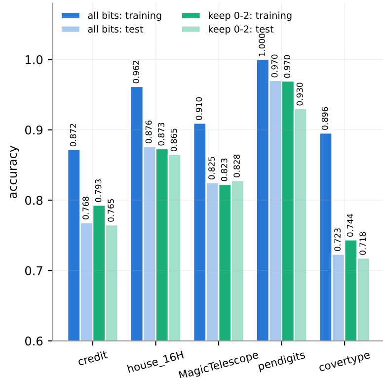
Accuracy on the classification datasets: training accuracy comes off the ceiling
