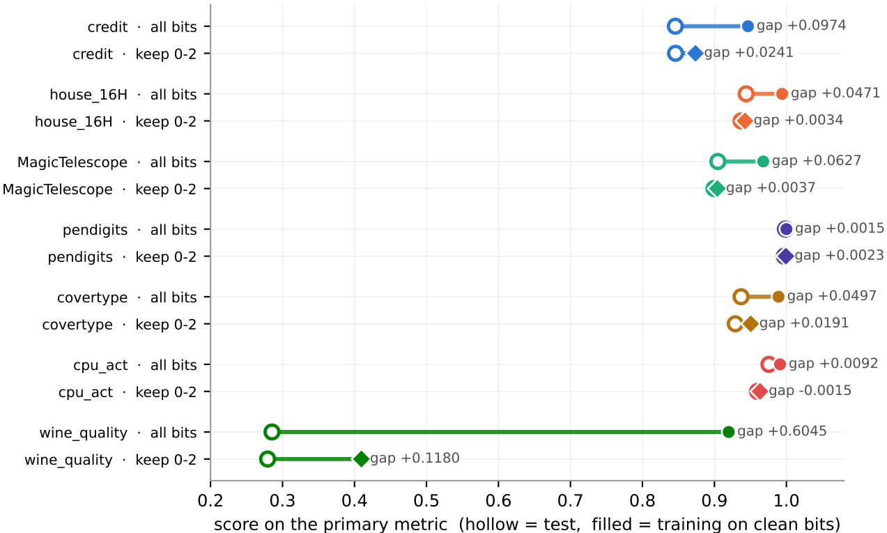
Training score falls toward the test score when the deep bits are removed
