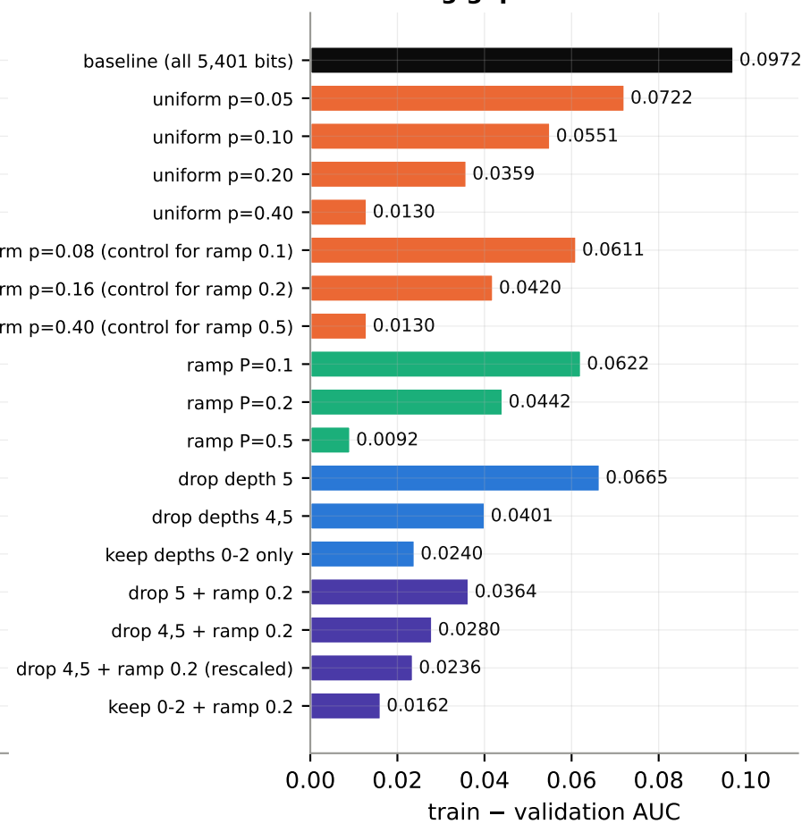
Overfitting gap
