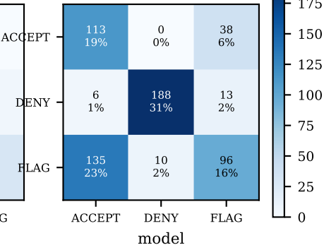
Structured CoT
