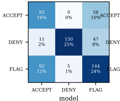
ground truth
