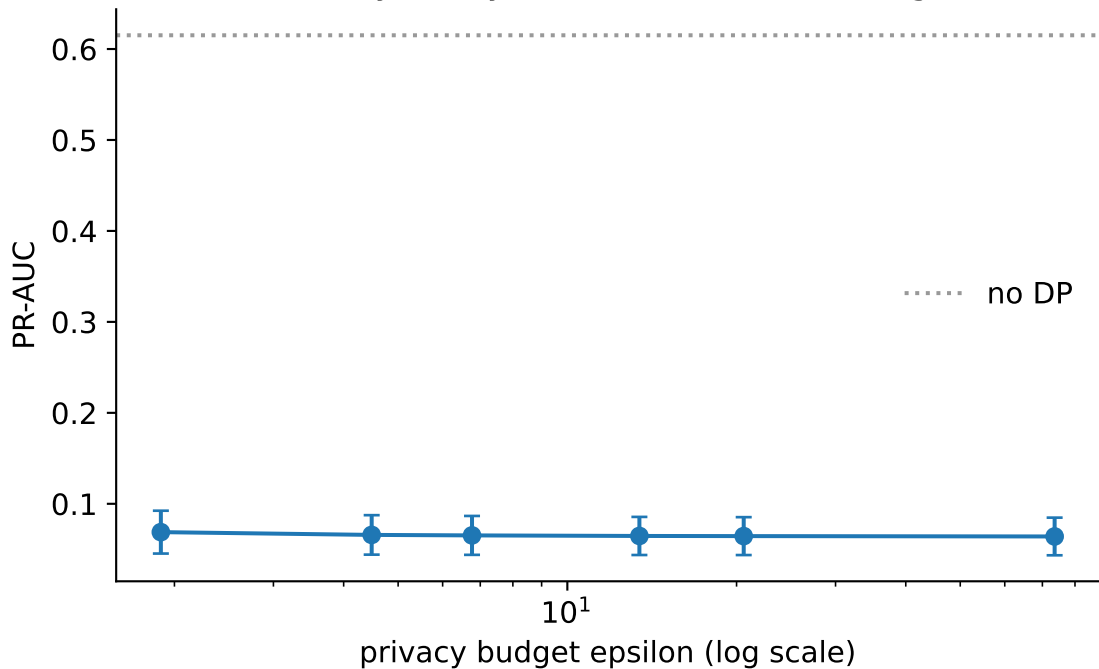
Privacy-utility trade-off (clean FedAvg)
