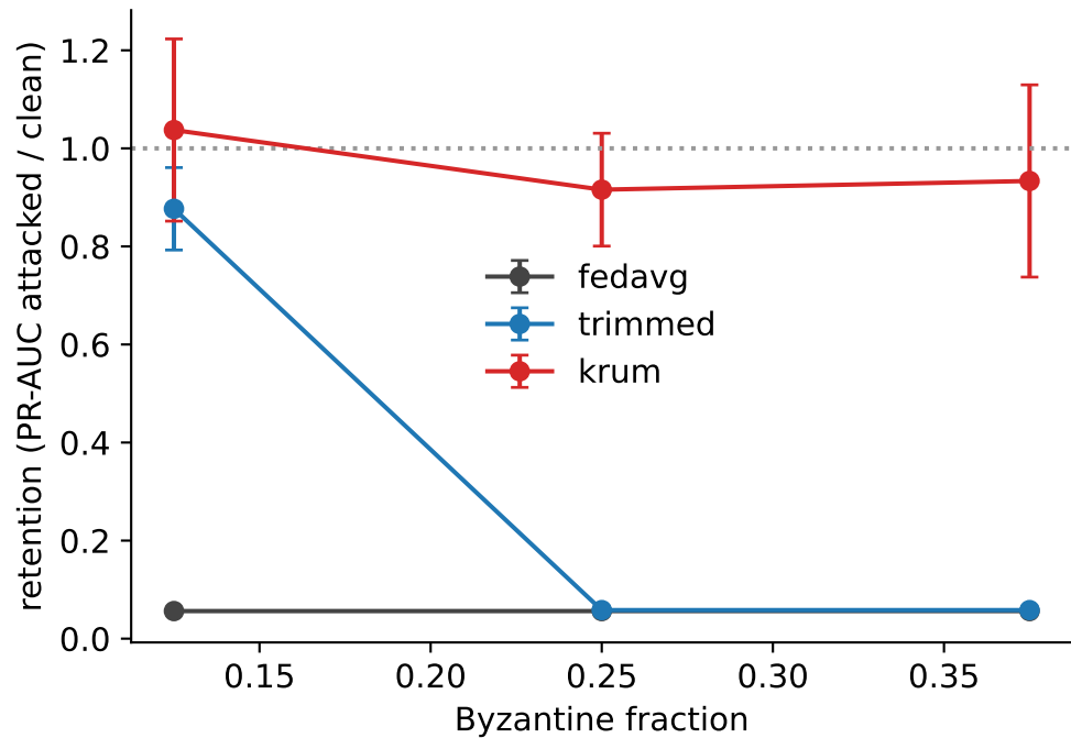
naive (boost)
